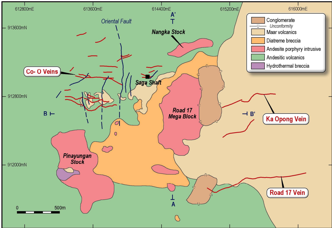
Figure 3. Co-O Mine area interpreted geological map showing section lines A-A' and B-B'.
