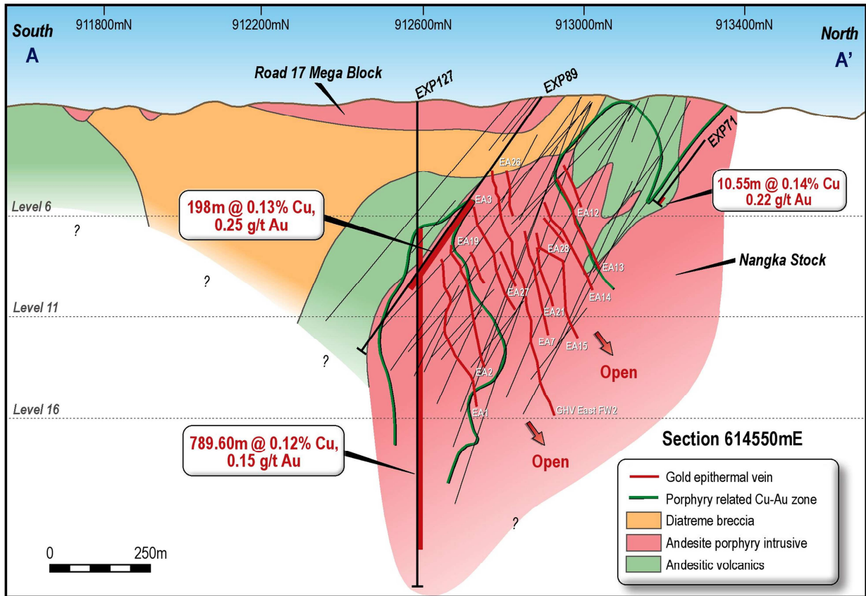
Figure 4. North-south cross section of the interpreted geology along section line A-A looking west.
