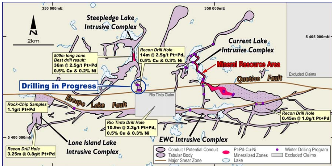
Figure 1. Intrusive complexes and the winter drilling program at Thunder Bay North.
