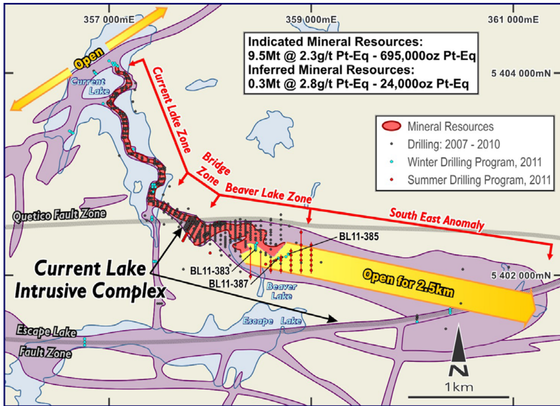
Figure 2. Summer drilling program in the Current Lake Intrusive Complex.
