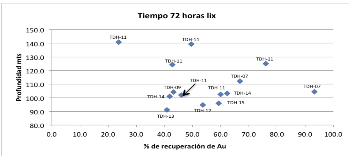
Primary Sulfide Zone Gold Recovery (% , horizontal axis) vs Depth (metres, vertical axis) after 72 Hours.
