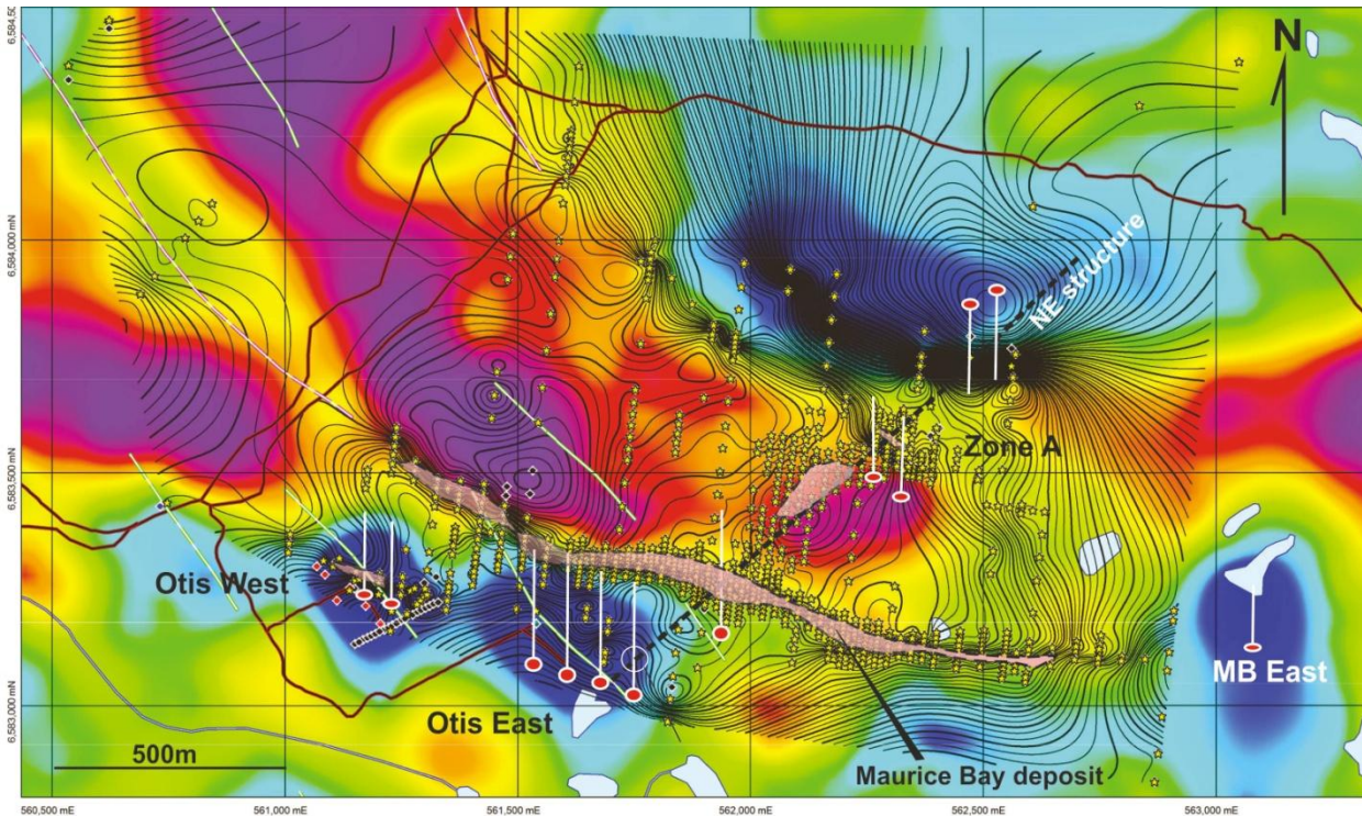
Figure 1: Map of Maurice Bay Deposit Area. Blue colours represent gravity lows, the reds are gravity highs, contours are depth to the unconformity. The uranium mineralization is in pink. Yellow dots are historical holes, most of which were stopped at the unconformity and red dots with white outlines are the proposed drill holes for 2014.
