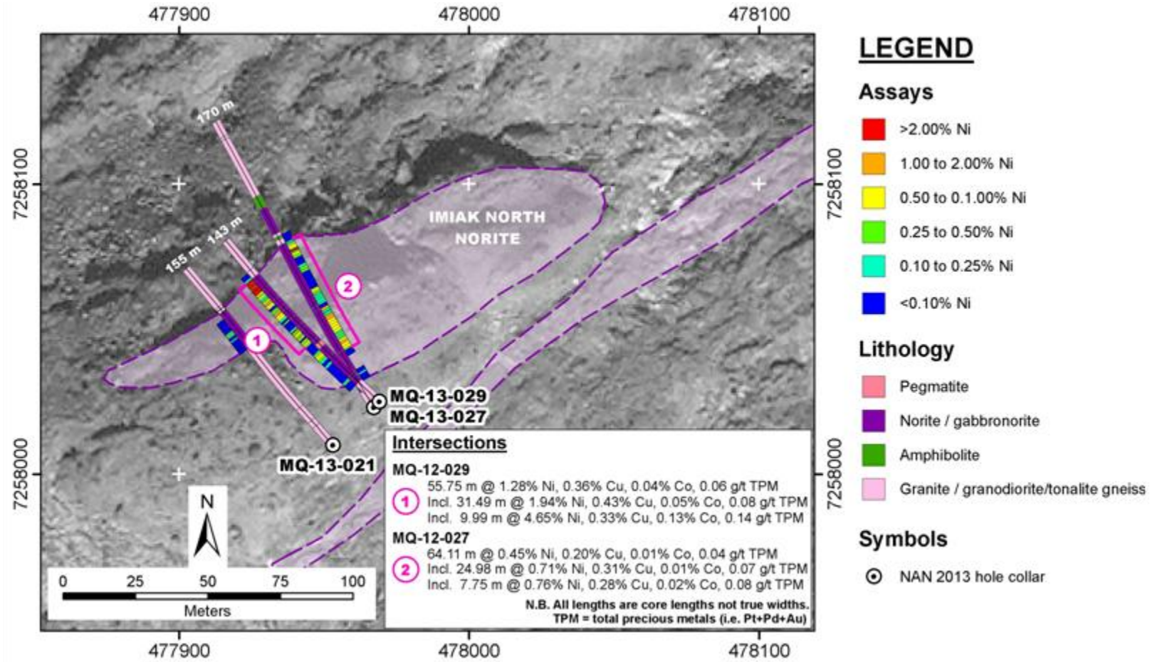
Figure 2: Imiak North Drill Plan
