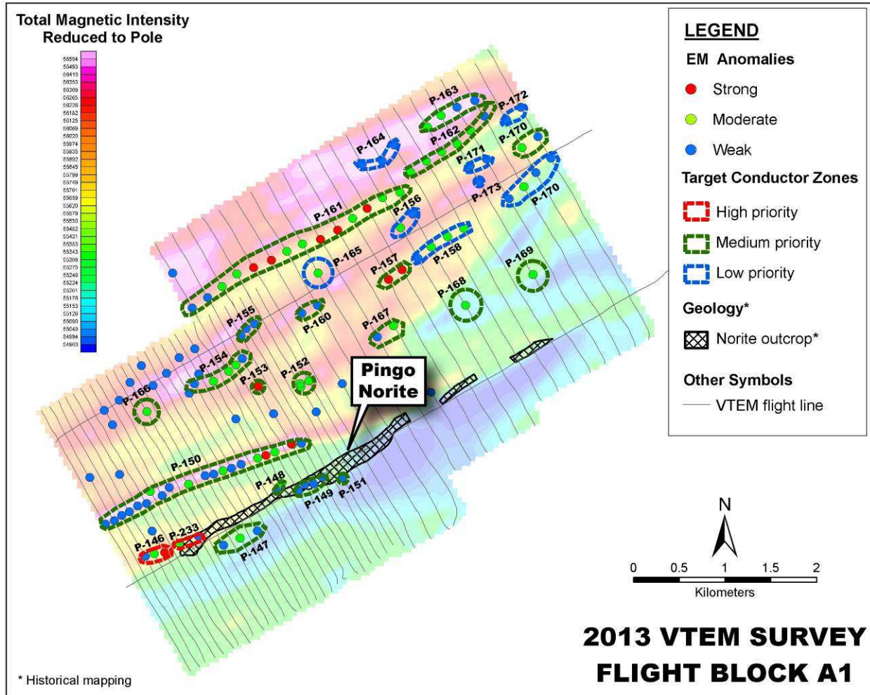
Figure 2: Map of 2013 VTEM survey block A1 showing electromagnetic anomalies, target conductor zones and total magnetic intensity reduced to pole.
