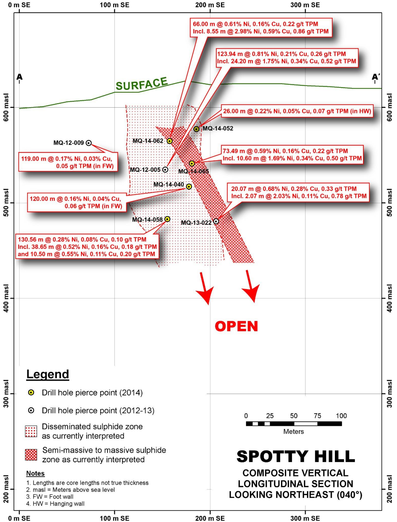
Figure 2: Composite vertical longitudinal section through Spotty Hill. The azimuth of the section is 130° and it looks N40°E. See Figure 1 for location.
