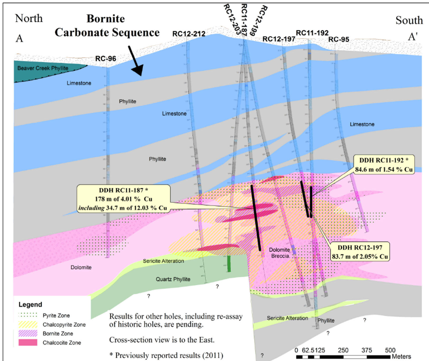
Figure 2: Cross-section through the South Reef Zone
