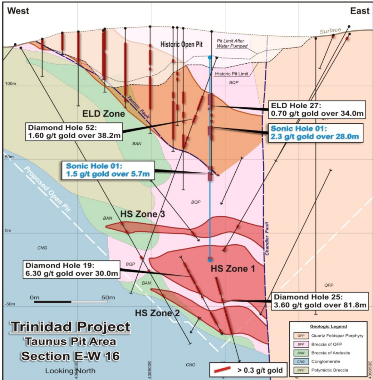
Figure 2. East-West section showing sonic hole 1 in Eldorado zone.
