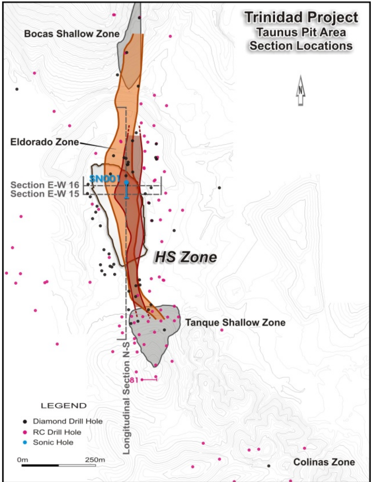
Figure 1. Plan map showing location of sonic hole 1 and sections.
