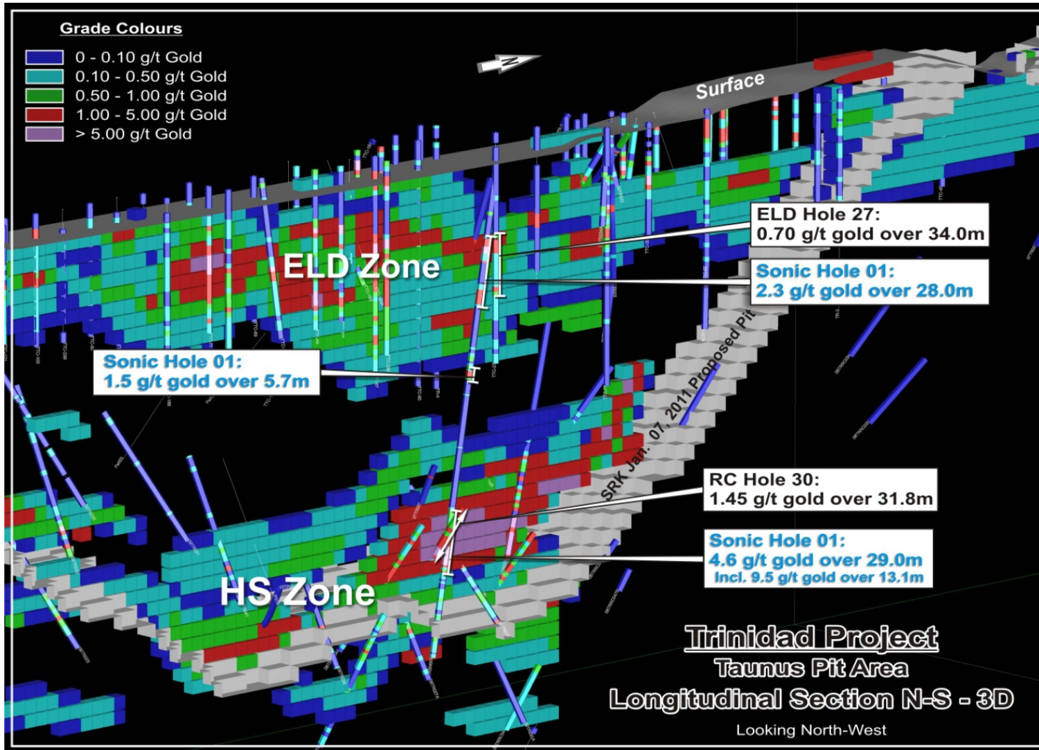
Figure 7. Three dimensional north-south longitudinal section showing sonic hole1 and block model.
