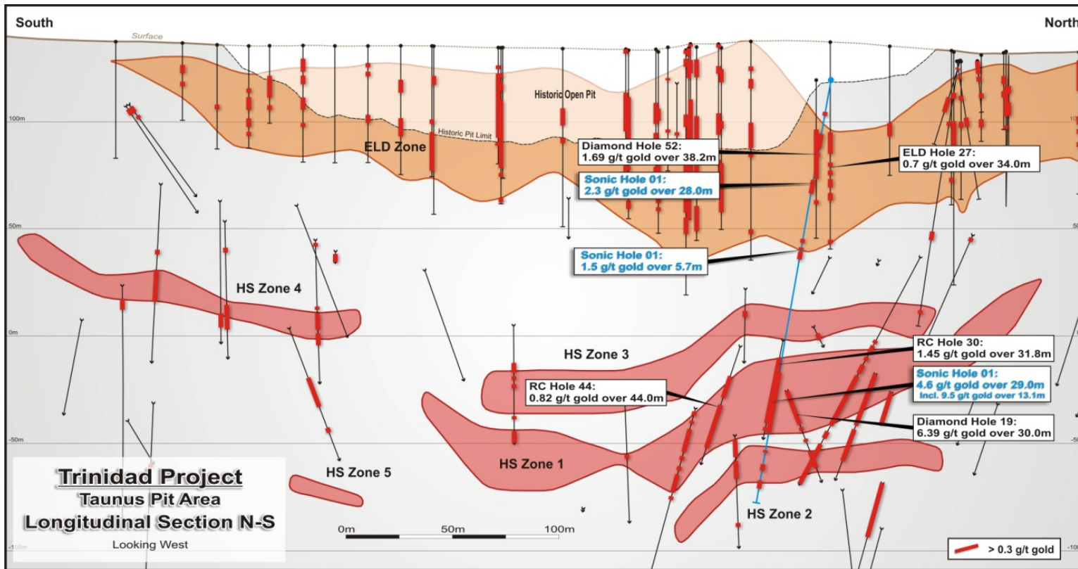
Figure 6. North-South longitudinal section showing sonic hole 1.
