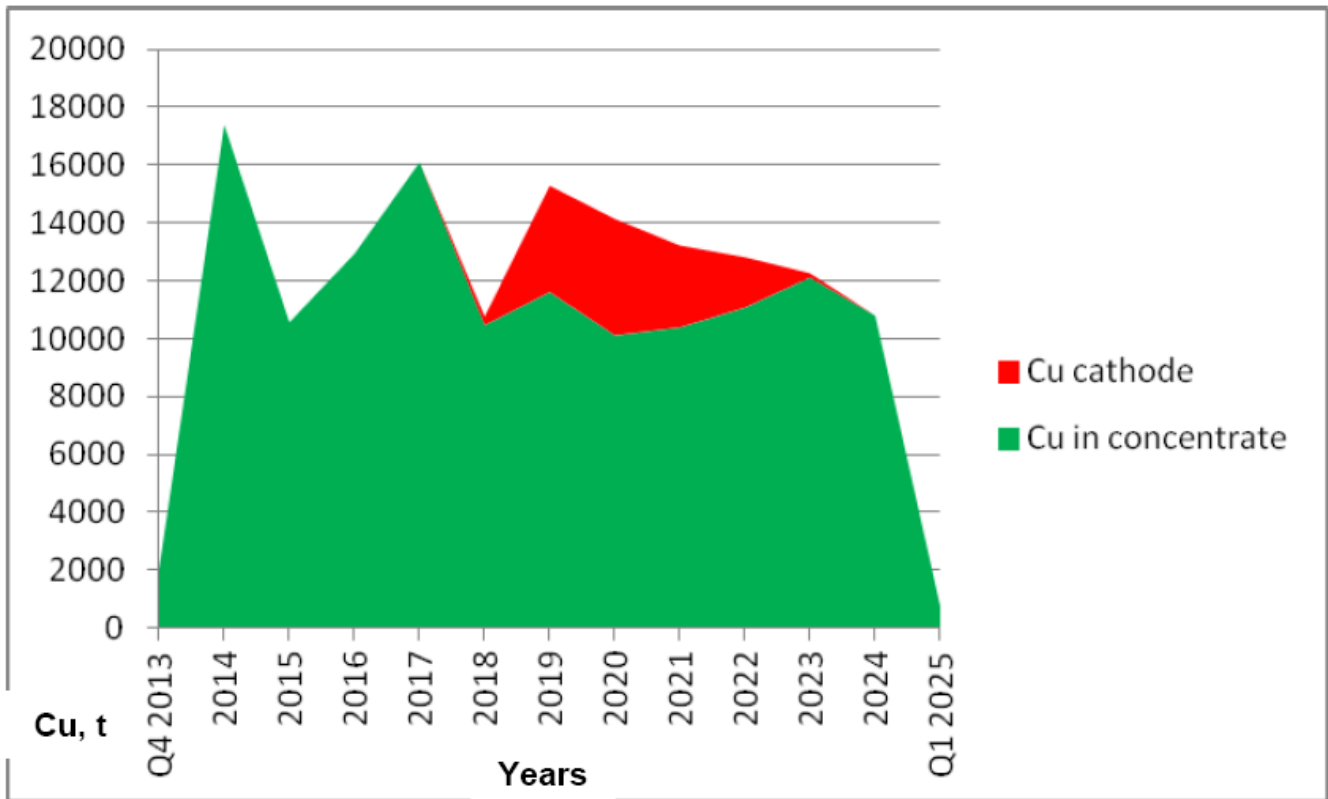
Figure 1. Production Profile of Copper in Concentrate and Cathode Copper.
