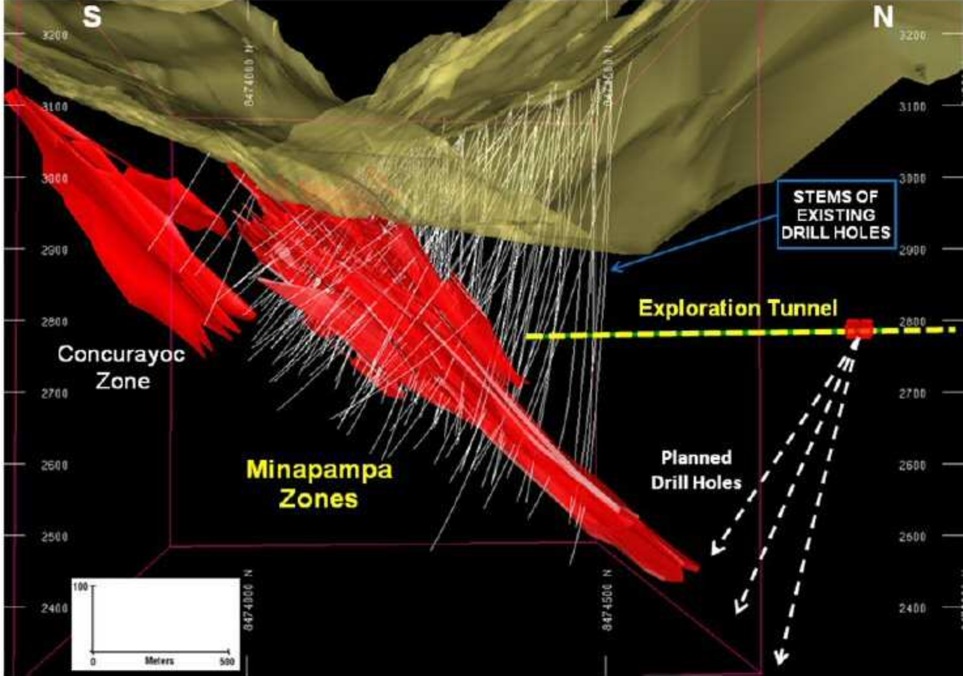
OLLACHEA PROJECT: 3-D CROSS-SECTION showing the topographic profile, a vertical & horizontal scale bar, the traces of existing drill stems (white), trace of the Challuno Exploration Access Tunnel (yellow), the Concurayoc and Minapampa Ore-bodies (red), and traces of programmed exploration extension drill holes (white)
