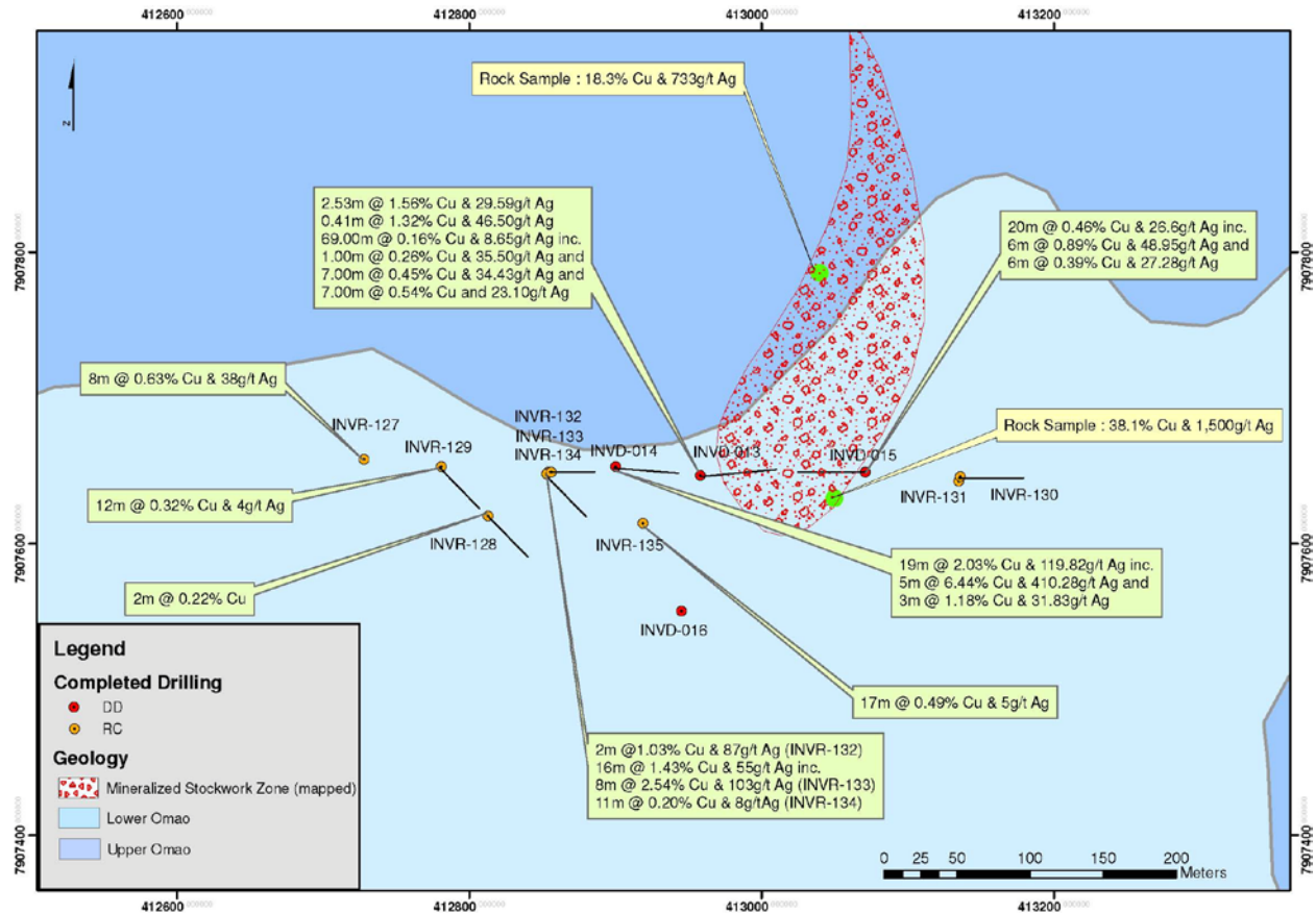
FIGURE 1: Omatapati Drill Plan and Geology
