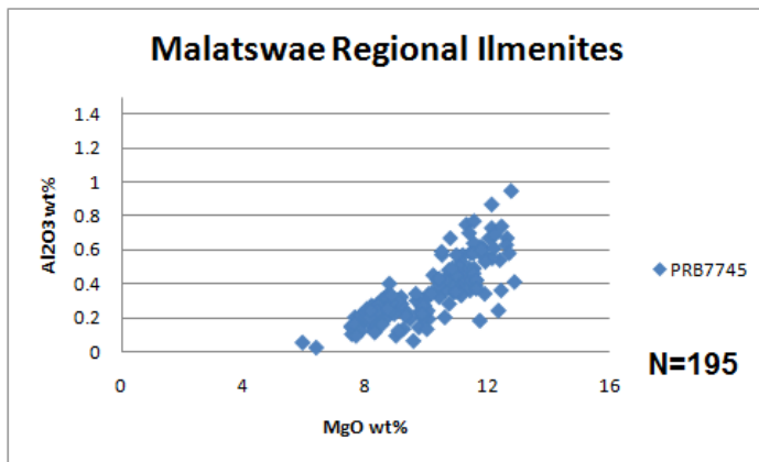
Figure 1: A comparison between the MgO - Cr 2 O 3 and MgO - Al 2 O 3 compositions of the ilmenites from the Malatswae Diamond Project Area and the Orapa AK1 diamond mine, Botswana.
