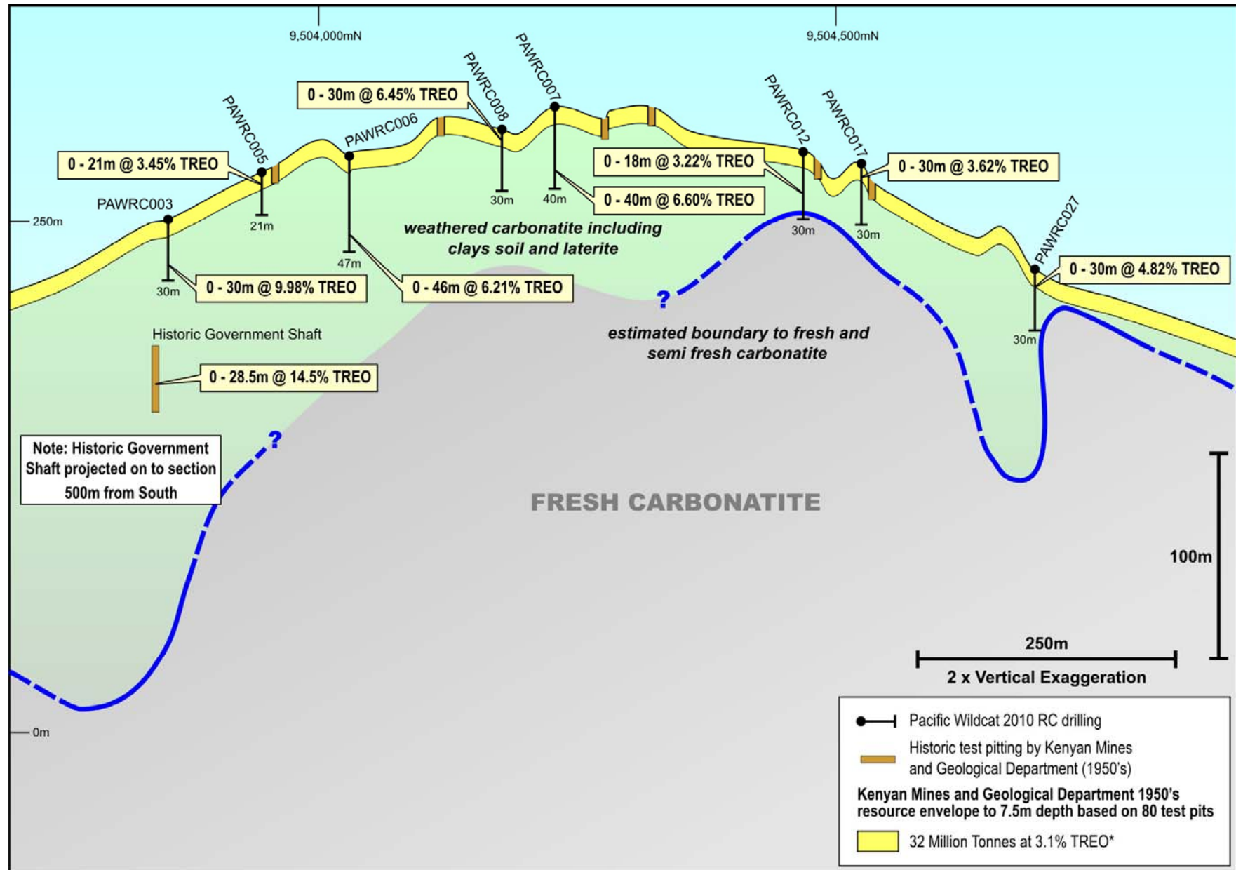
Figure 2: Conceptual Cross Section Showing Rare Earth Intersections
