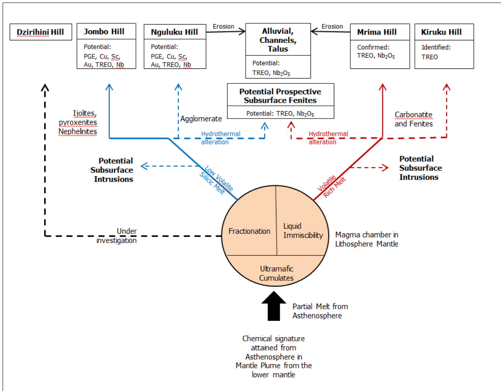
Figure 3: Genesis of the intrusive alkaline igneous rocks, and prospectivity of the Mrima Hill Area. Adapted from K. Collerson's internal PAW report (2012).
