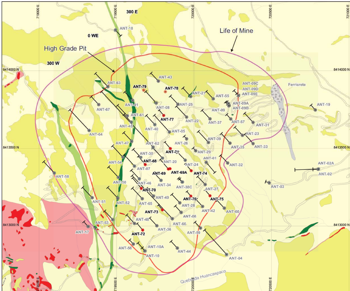
Figure 1 ANTILLA COPPER PROJECT EAST BLOCK GEOLOGY AND DRILL HOLES
