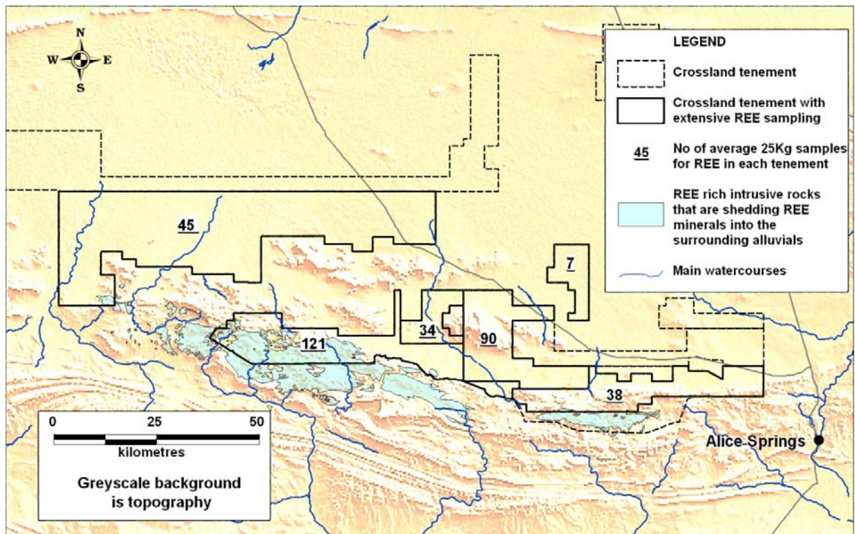
Fig 2: Charley Creek Project Tenements showing REE bearing rocks, topography, and number of stream sediment samples collected from each title as at Feb 28, 2011. Each sample is from 2 to 4 square kilometres of drainage basin. Total number collected: 335.
