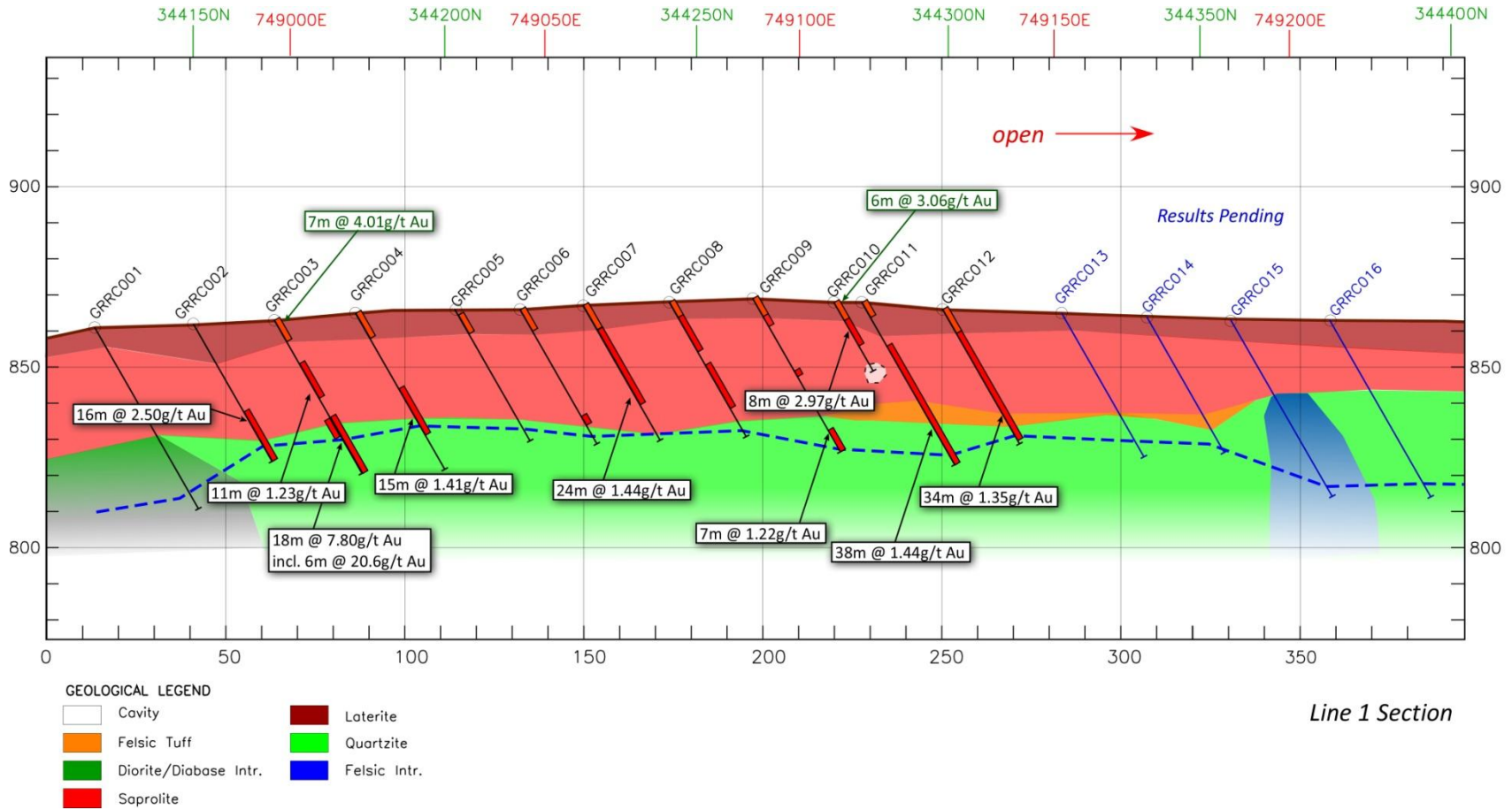
Figure 2: Section across Line 1 showing the lithology and main mineralised intervals
