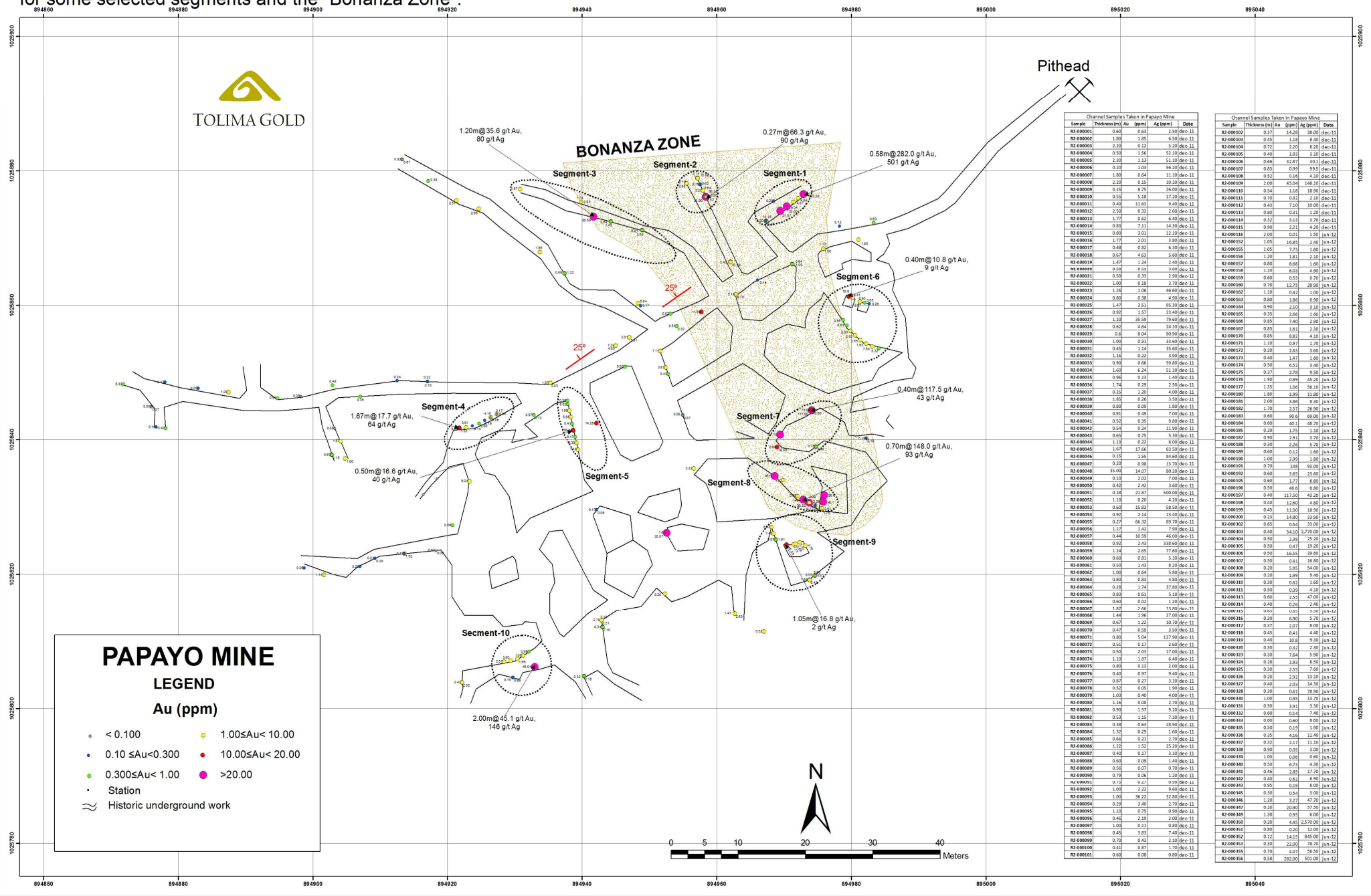
Figure 1: Plan view of the El Papayo mine showing drift and underground cross-cuts sampling colour-coded for gold grades, data from highest grade gold samples for some selected segments and the "Bonanza Zone".
