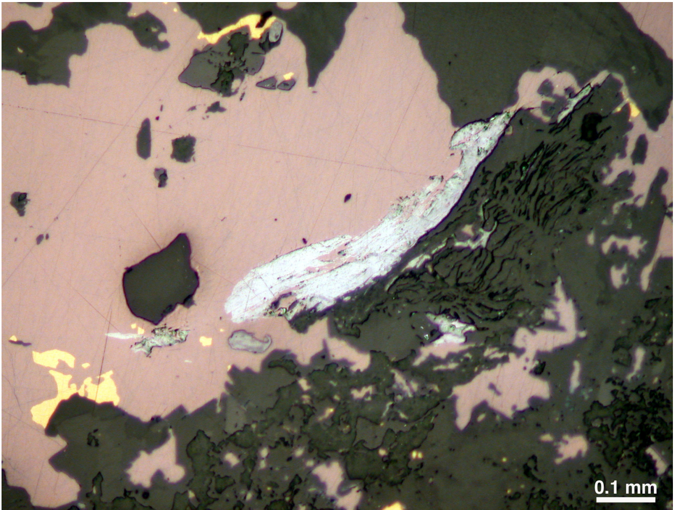
Molybdenite (silver) in bornite intergrown with chalcopyrite (yellow) and gangue (carbonate, sericite). FOV = 0.86 x 1.15 mm.
