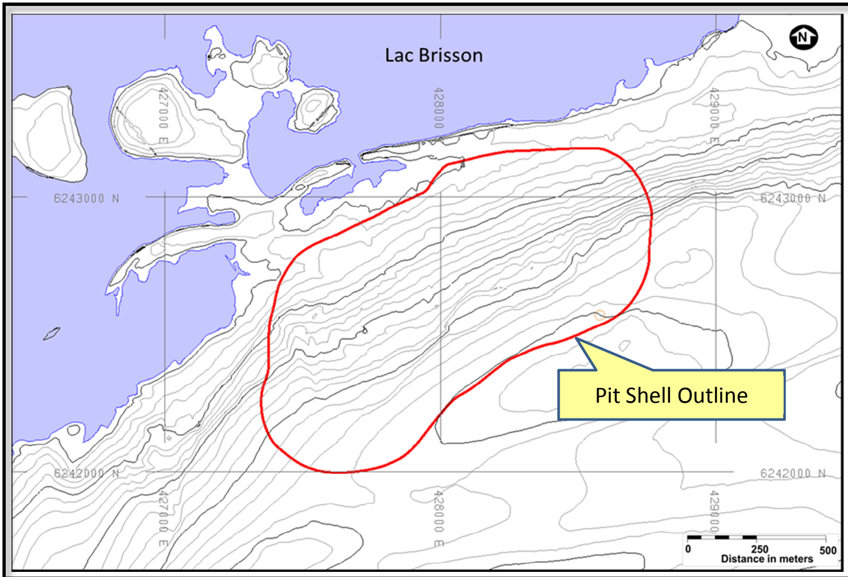
Figure 1 – Outline of the Whittle Pit Shell Used in the Resource Estimation, B-Zone REE Deposit, Strange Lake Project, Québec
