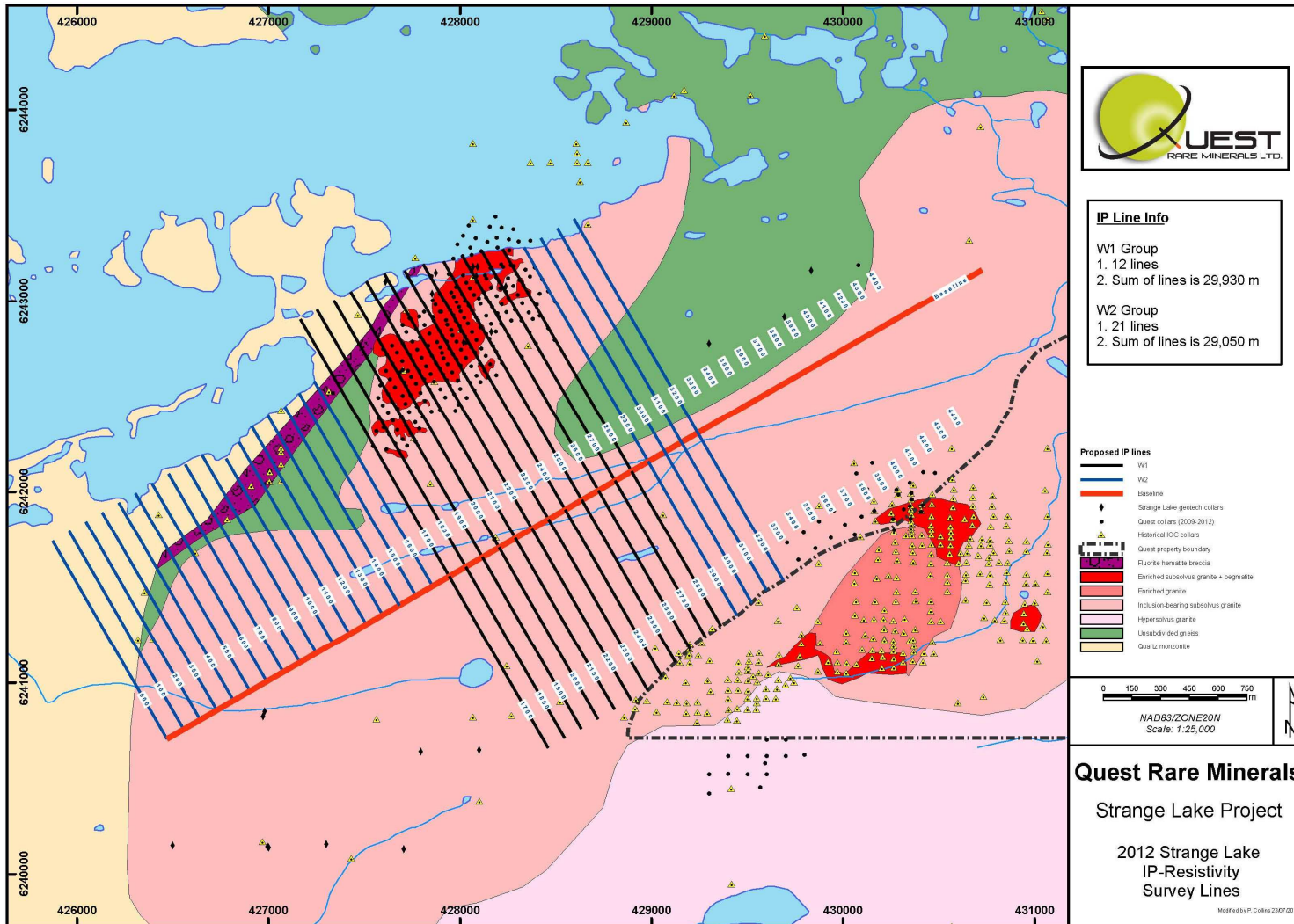
Figure 4 – Geophysical Survey Plan Map, Strange Lake Project, Québec
