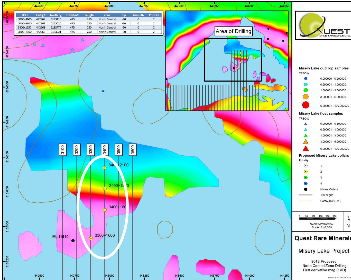
Figure 6 – North Central Drilling Location Map, Misery Lake Project, Québec
