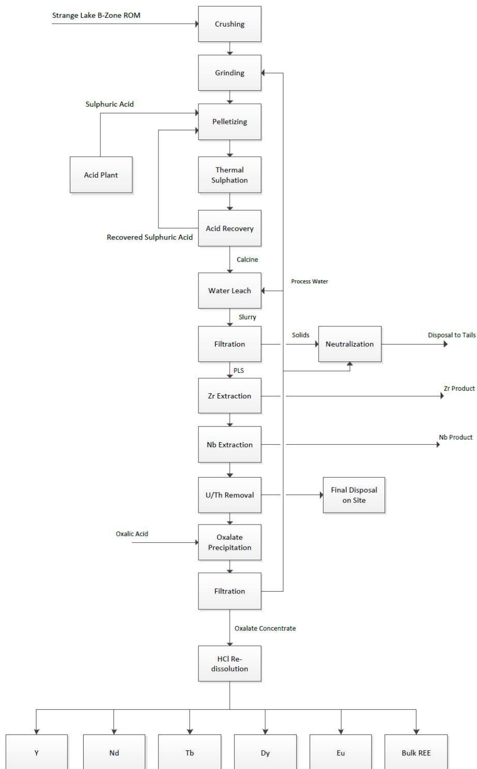
Figure 1 - Block Flow Diagram
