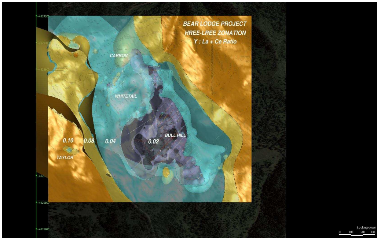
Figure 2. LREE-HREE zonation in the Bear Lodge REE district as expressed by the abundance ratio of Y/La+Ce.
