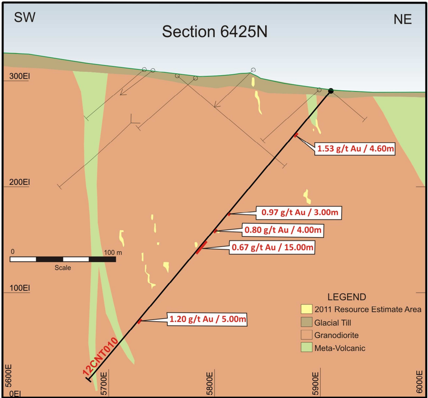
Figure 3 - Cross Section 6425N
