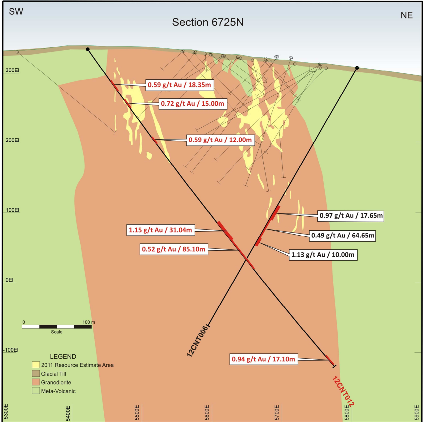
Figure 4 - Cross Section 6725N
