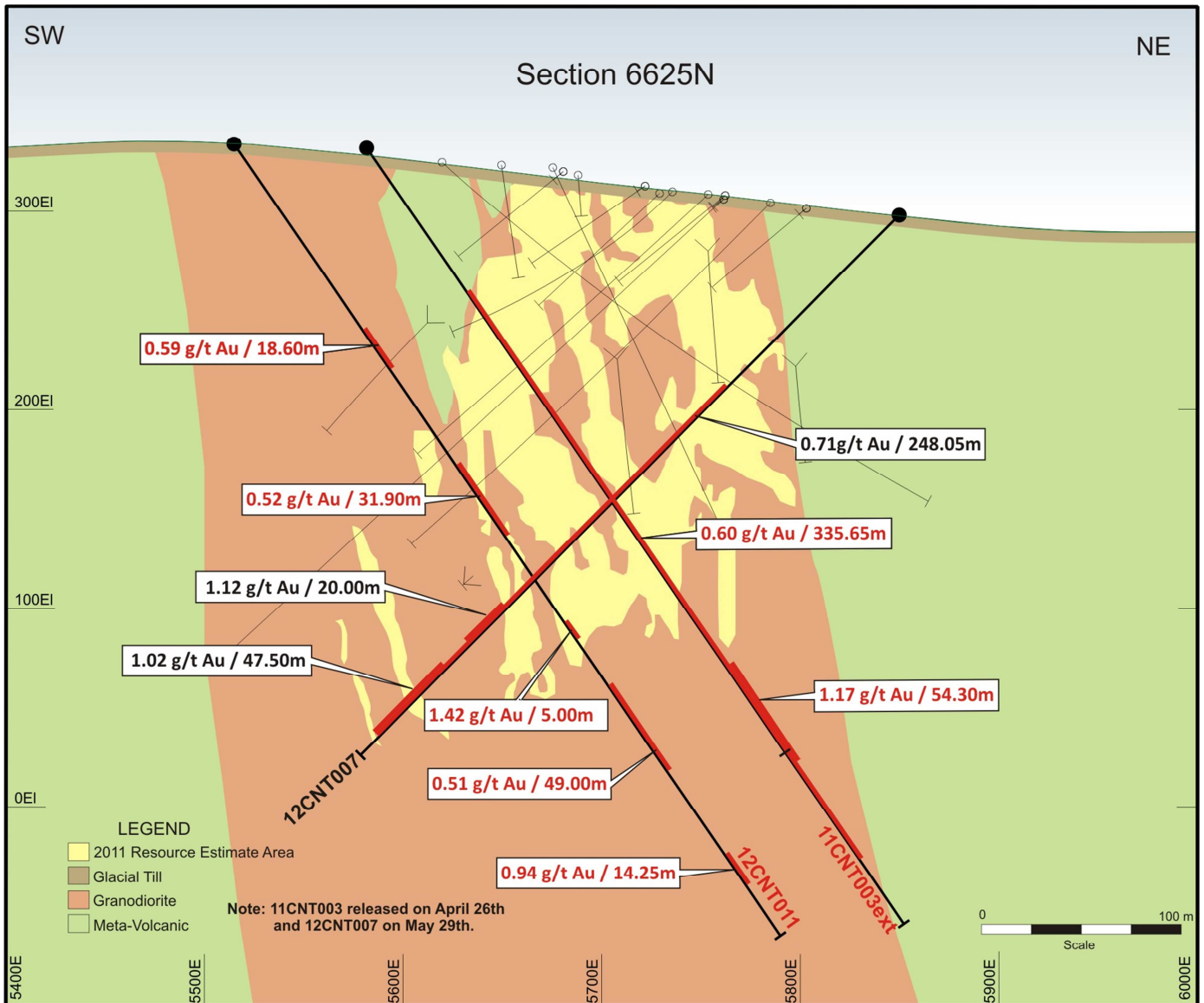
Figure 1 - Cross Section 6625N
