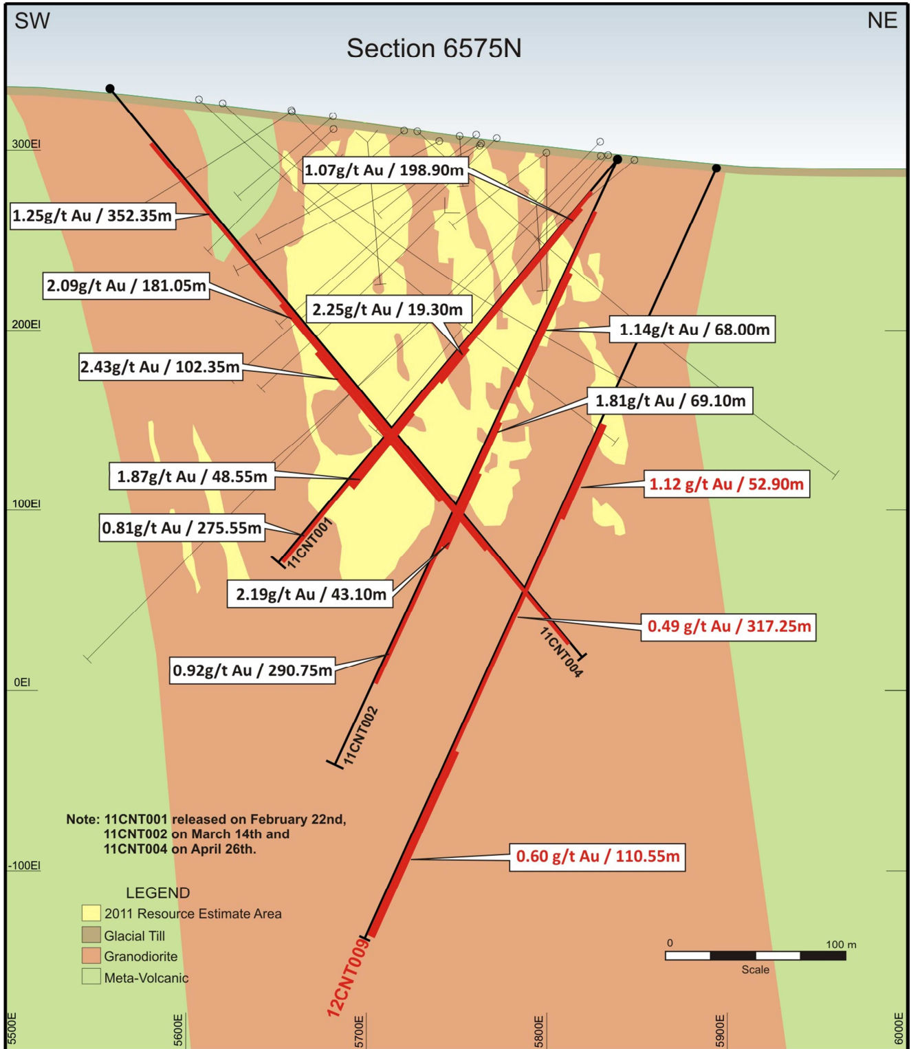
Figure 2 - Cross Section 6575N
