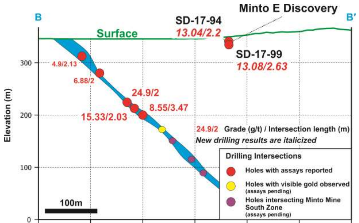
Figure 3. Cross-section showing the spatial relation between the Minto Mine South Zone and the discovered high-grade quartz vein
