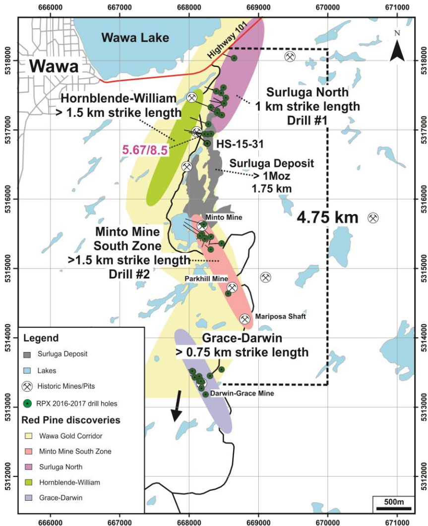
Figure 1. Red Pine's discoveries and 2016-17 drilling overview
