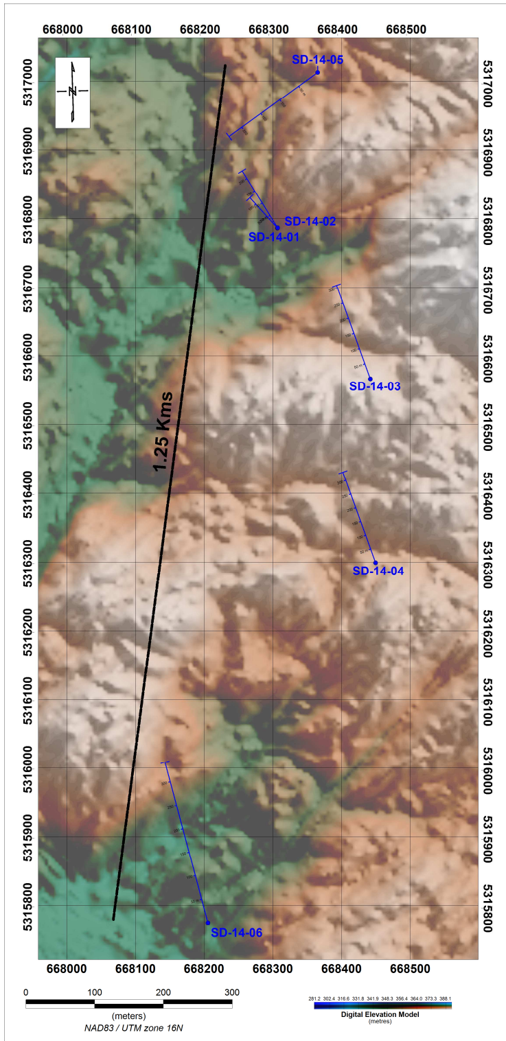
Figure 1. Digital Elevation Model (DEM) map showing the location of the December 2014 Drill Holes
