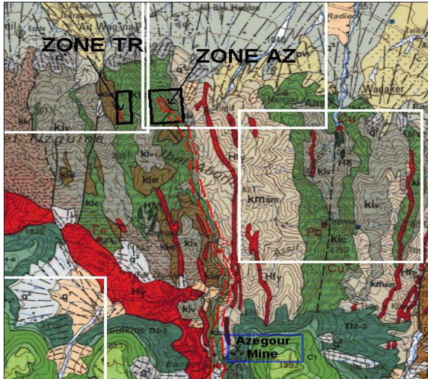
Figure 1: Regional geology map showing the location of the AZ and TR Zones relative to the Azegour Mine and the NNW mineralized trend identified by Permigeat (1957).
