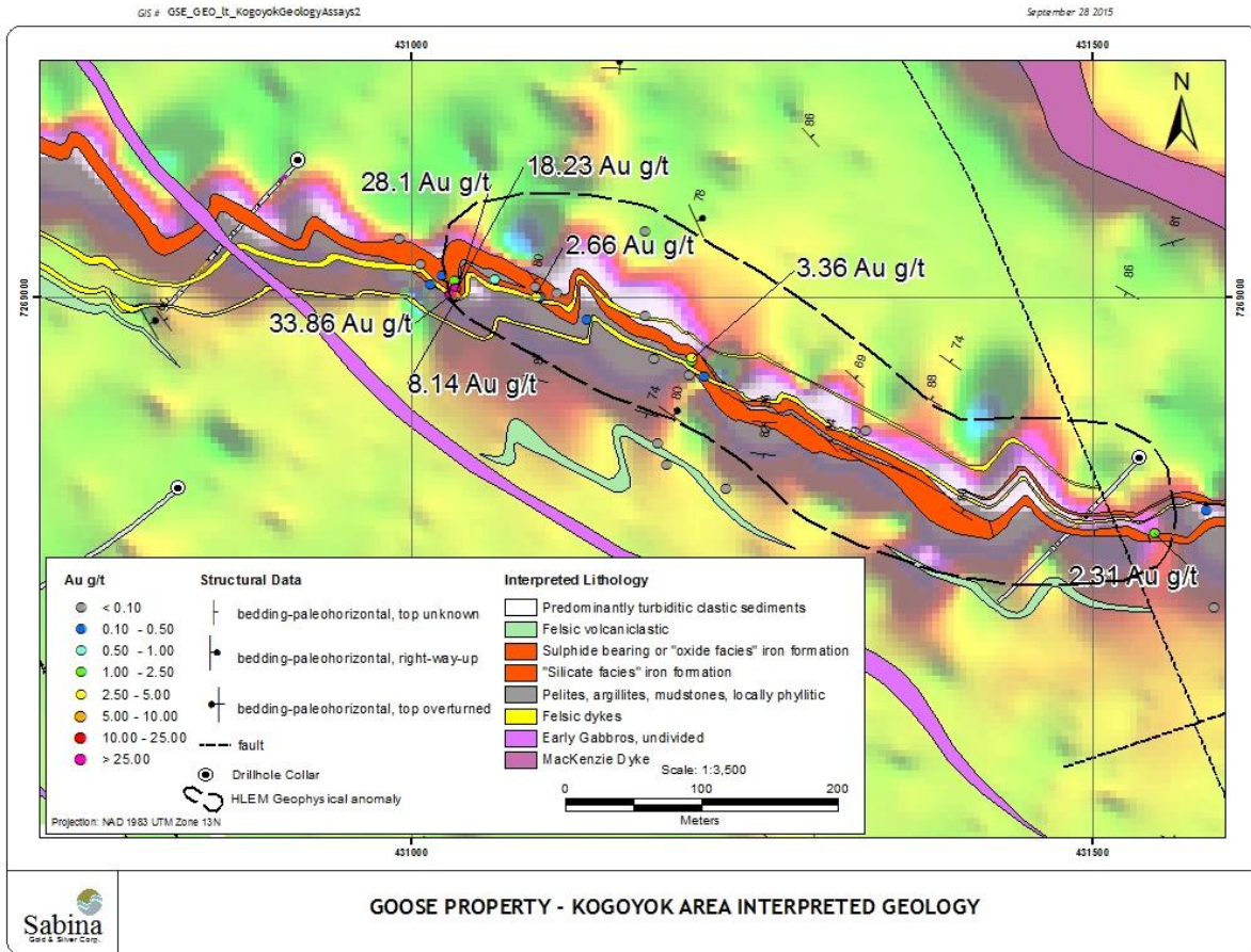
Figure 2. Kogoyok interpreted geology map with select assay values.
