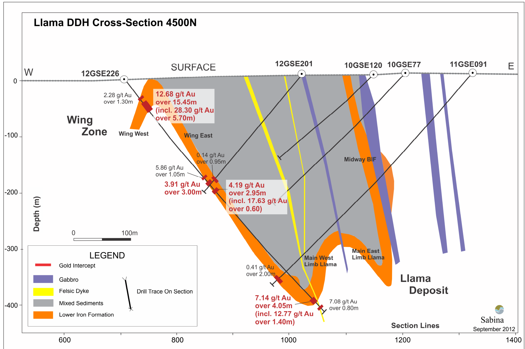
Figure 3: Llama 4500N Cross Section
