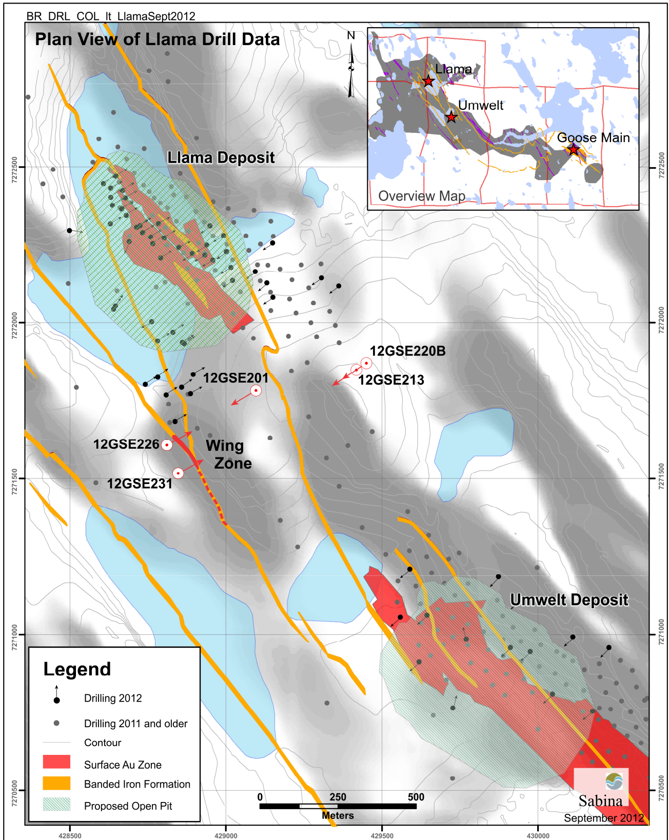
Figure 1: Plan View of Llama, Umwelt and Wing Zone Drilling
