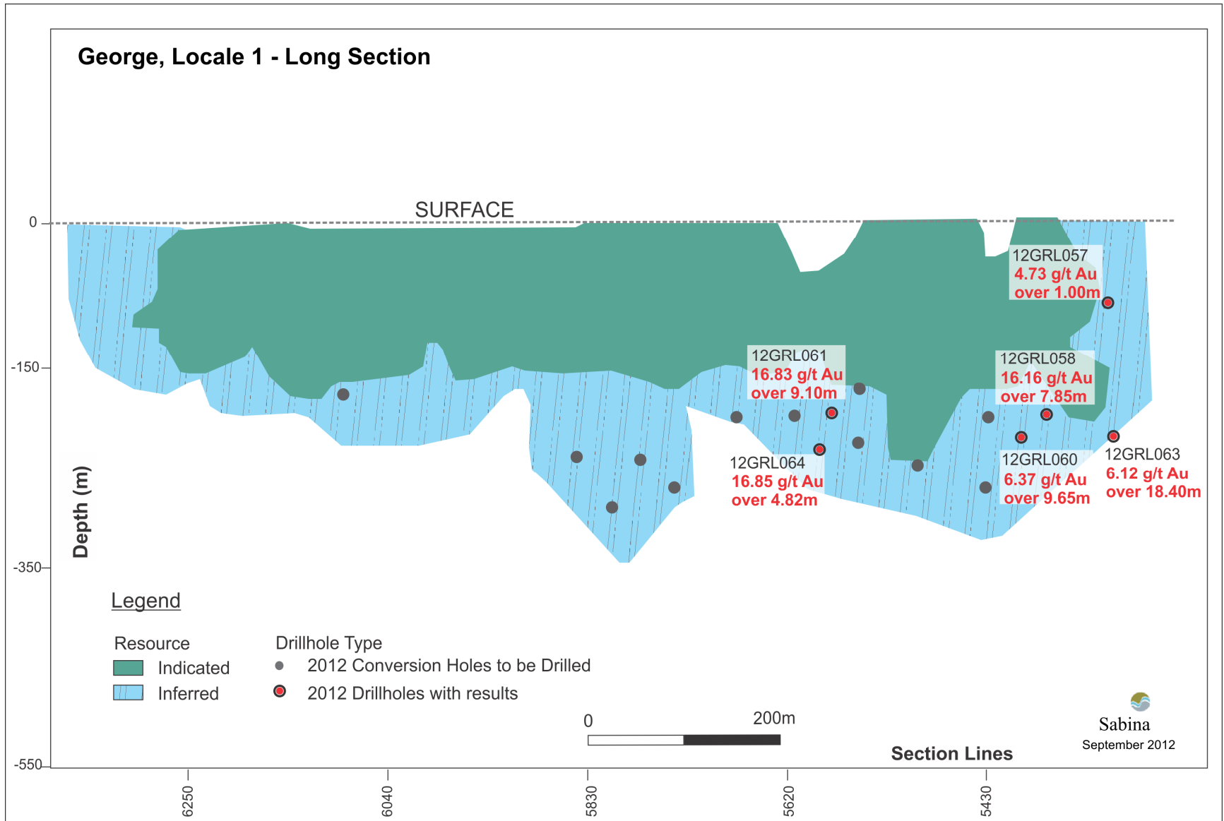
Figure 4: Locale 1 Long Section
