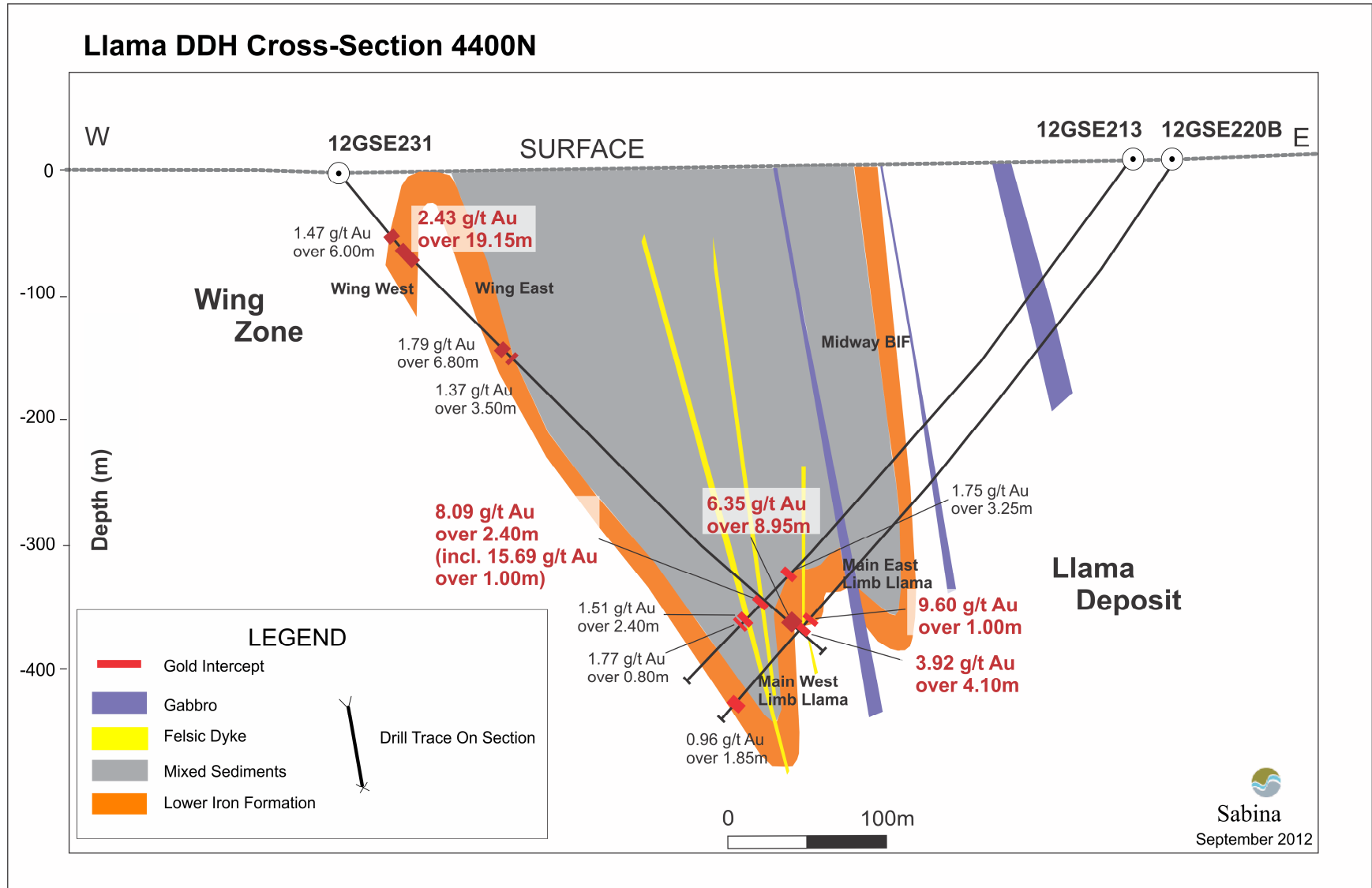
Figure 2: Llama 4400N Cross Section
