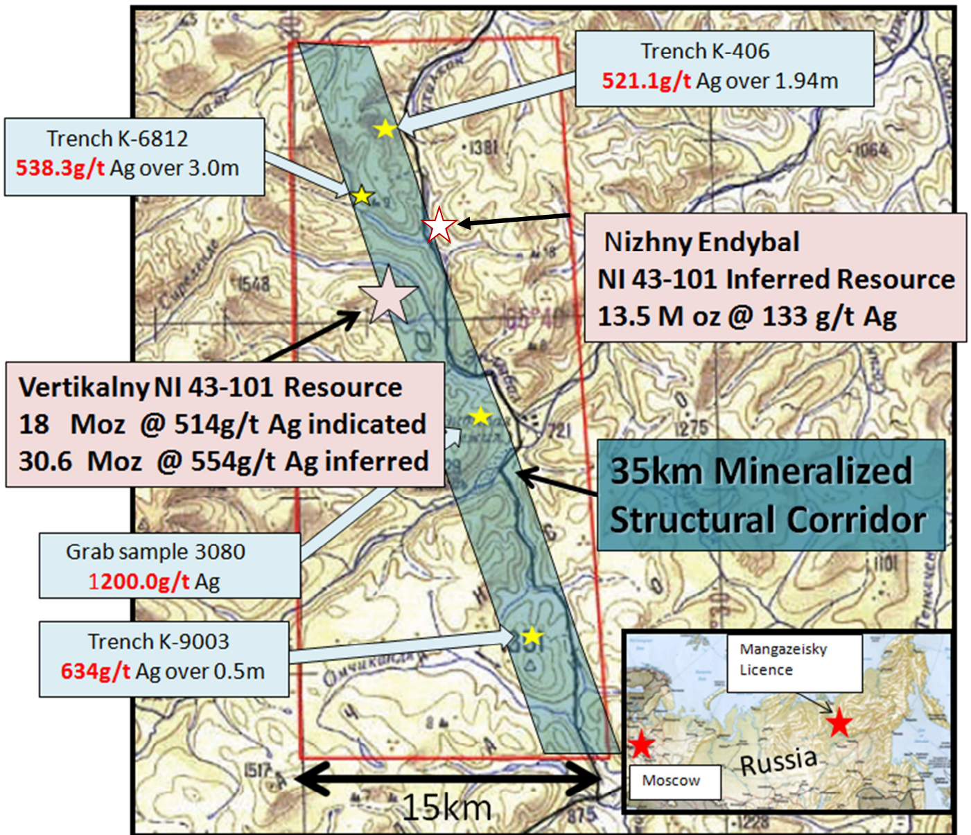
FIGURE 1: MANGAZEISKY LICENCE SHOWING VERTIKLANY RESOURCE AND HISTORICAL INTERCEPTS
