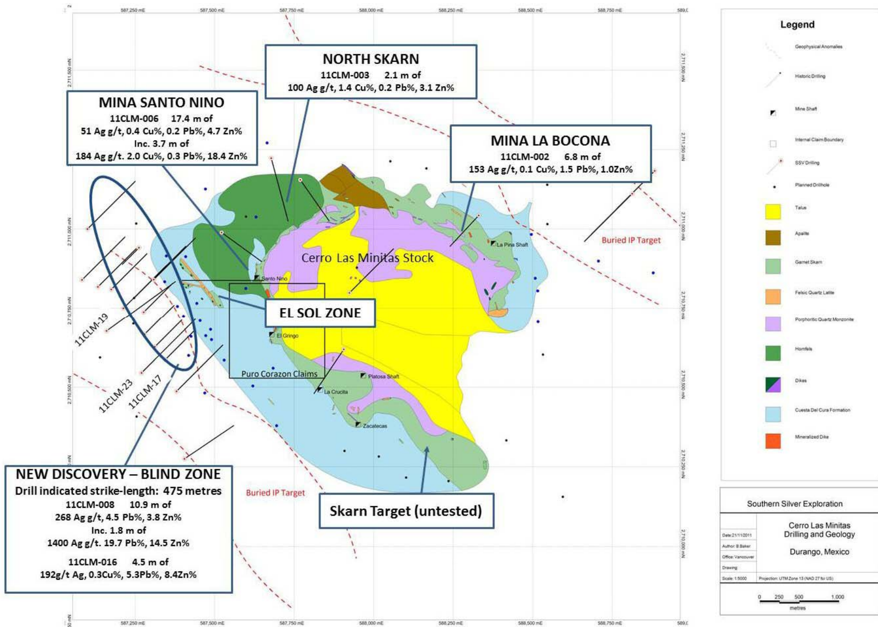
Figure 1: Drill Hole Distribution and Significant Targets – Cerro Las Minitas
