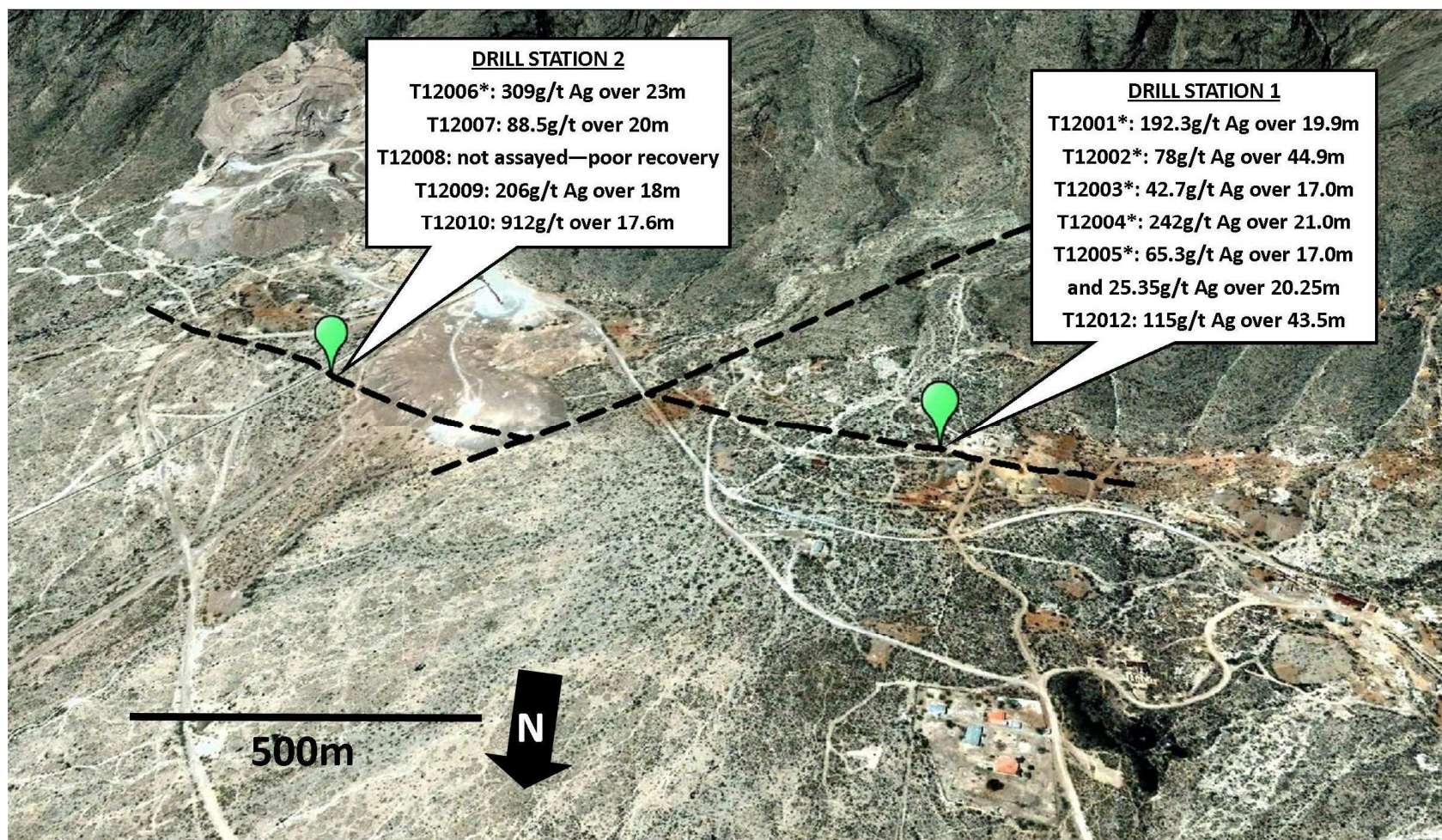
Figure 2. The locations of the first two underground drill stations in relation to map structures at the eastern end of the Shallow Silver Zone. The high grade silver mineralization is hosted along east-west striking structures that are traceable for over 1 kilometer. (* refers to drill holes previously reported)
