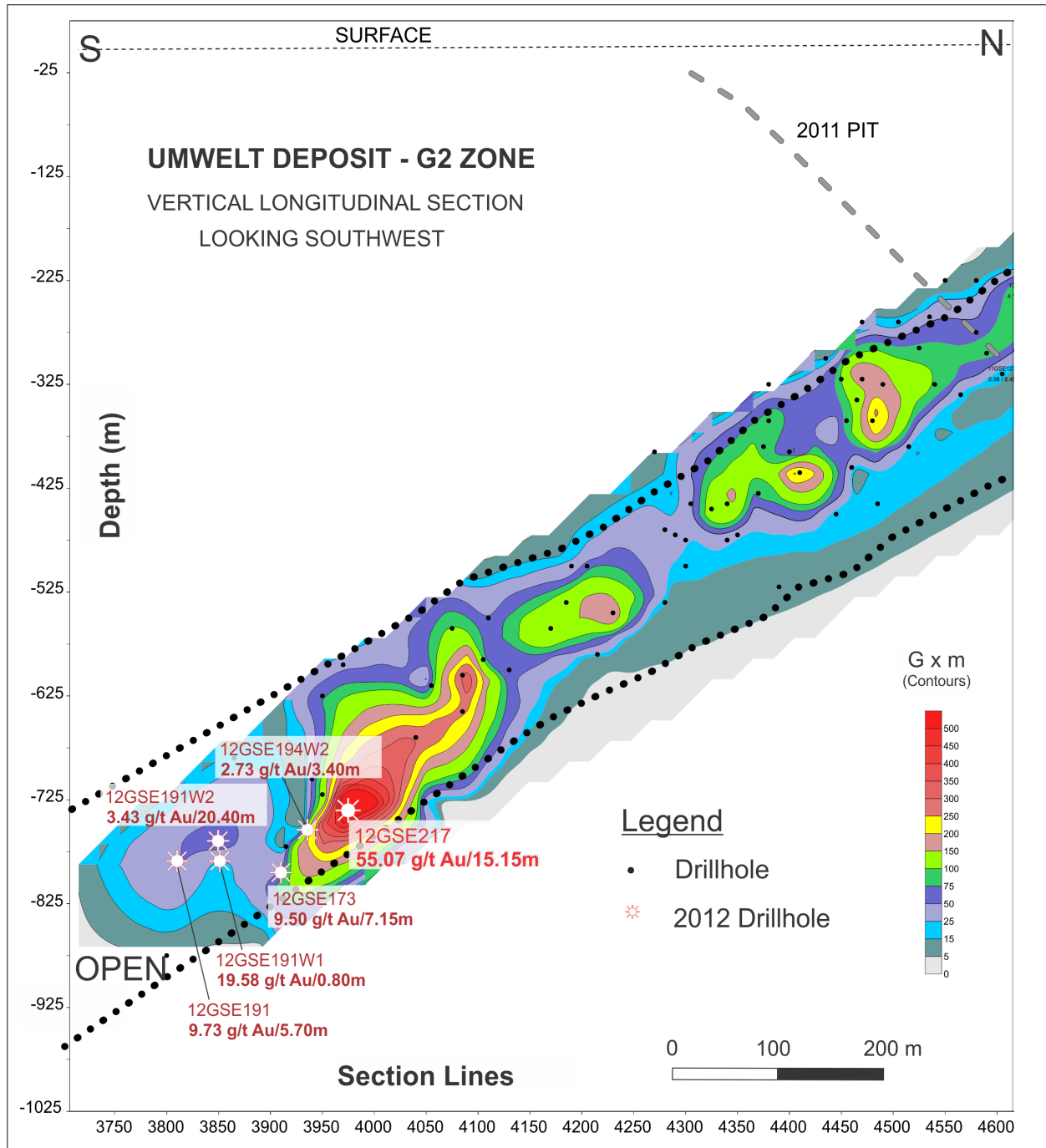
Figure 2: Umwelt Long Section 217 clipped
