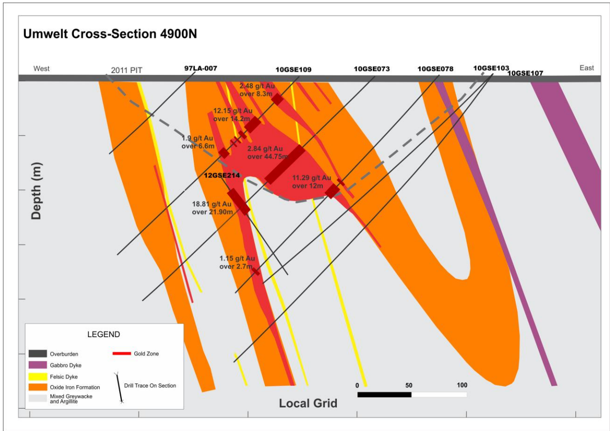
Figure 1:Umwelt Cross Section 214
