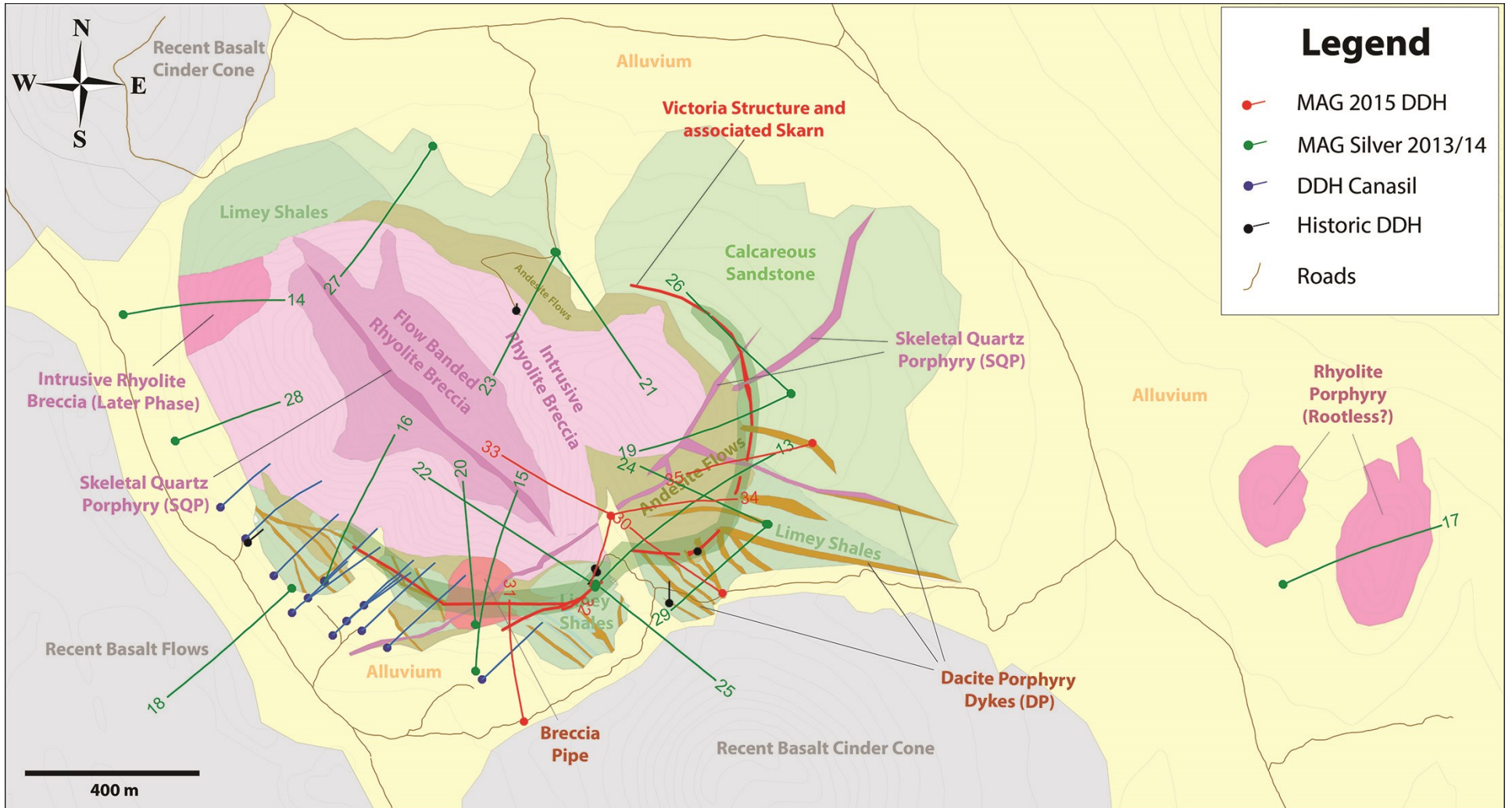
Figure 1: Simplified Geological Map of the Salamandra Property
