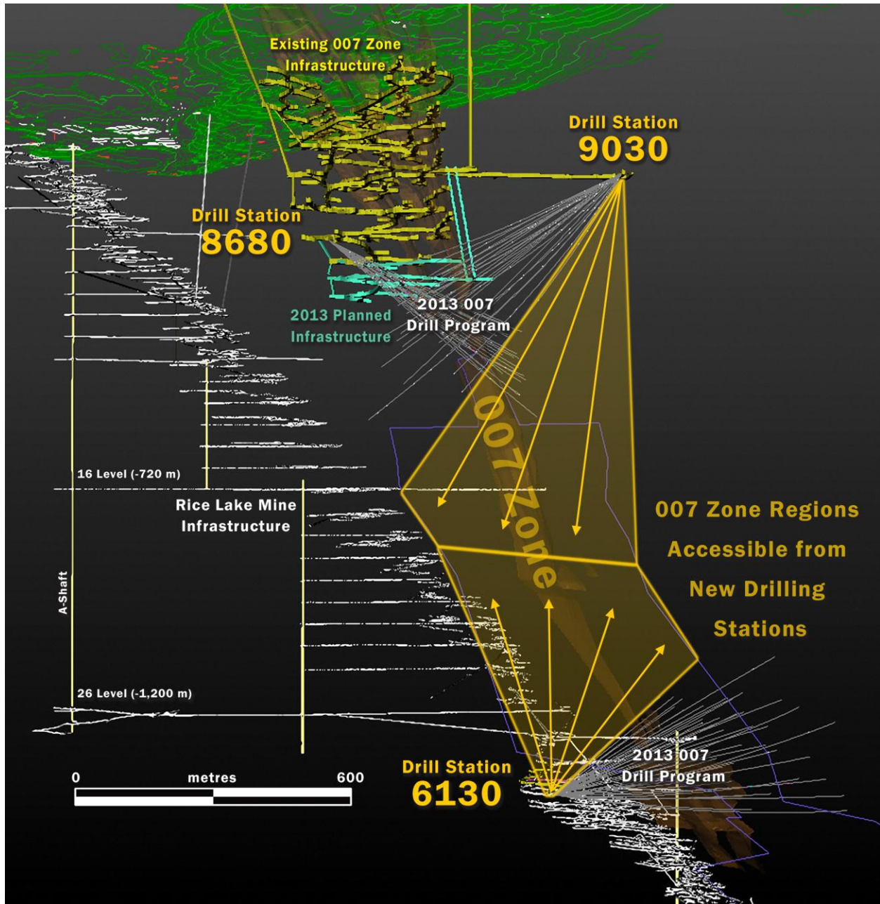
Figure 2: 007 Zone Regions Accessible from 9030 and 6130 drilling stations.
