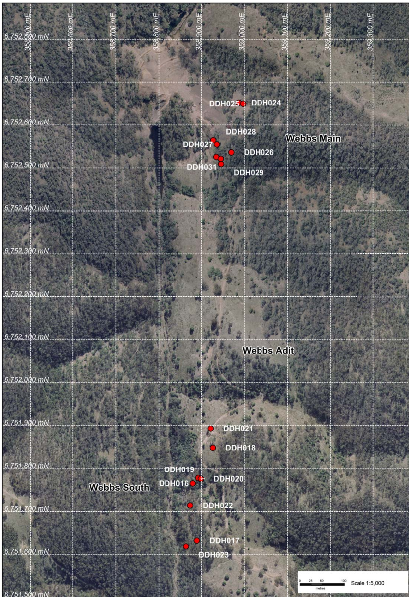
Figure 3 - Webbs Silver Project 2011 DDH Locations
