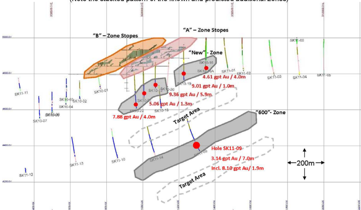
Figure 2: North Diorite Longitudinal Section (Facing North) – Simkar Project Projected drill holes are from 2010 and 2011 exploration campaigns only (Note the stacked pattern of the known and predicted additional zones)
