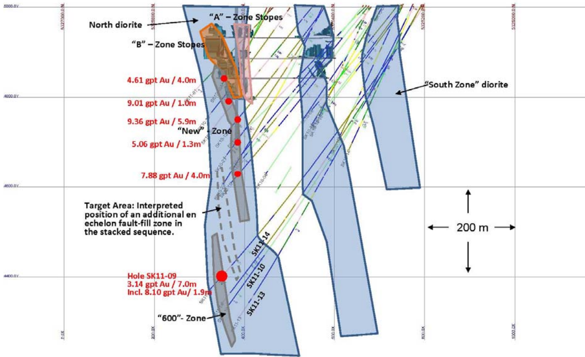
Figure 1: Composite Cross Section (Facing East) – Simkar Project Projected drill holes are from 2010 and 2011 exploration campaigns only
