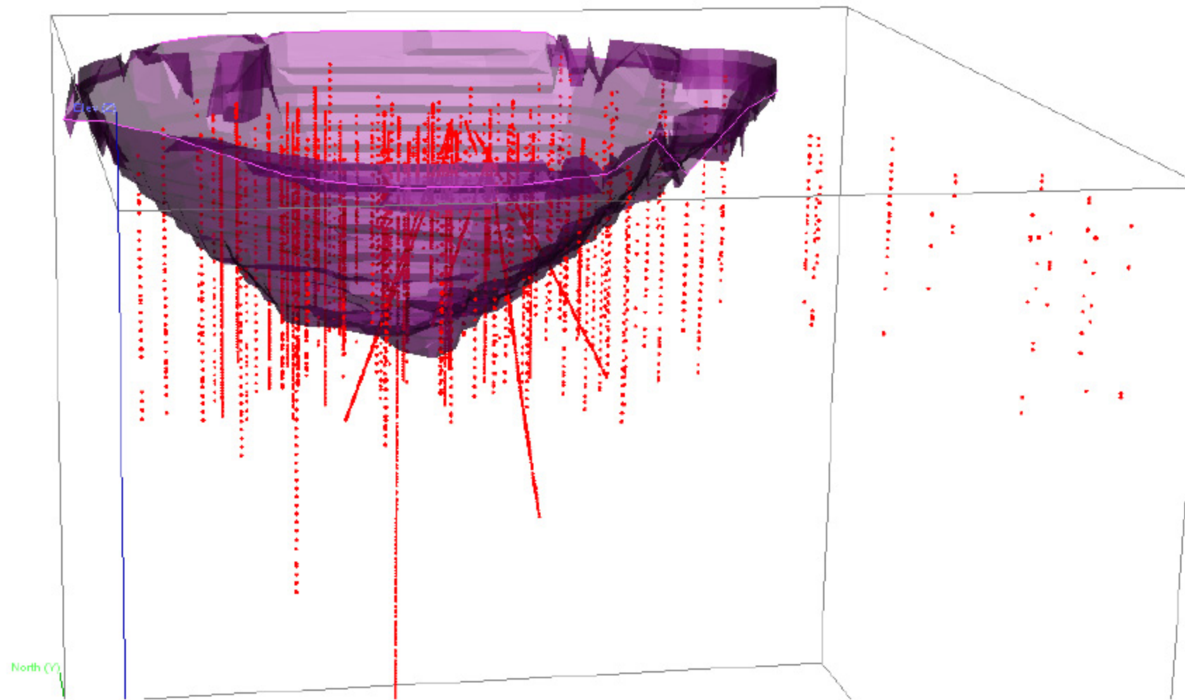
Figure 1: Gold and silver only assay data 3D view looking north
