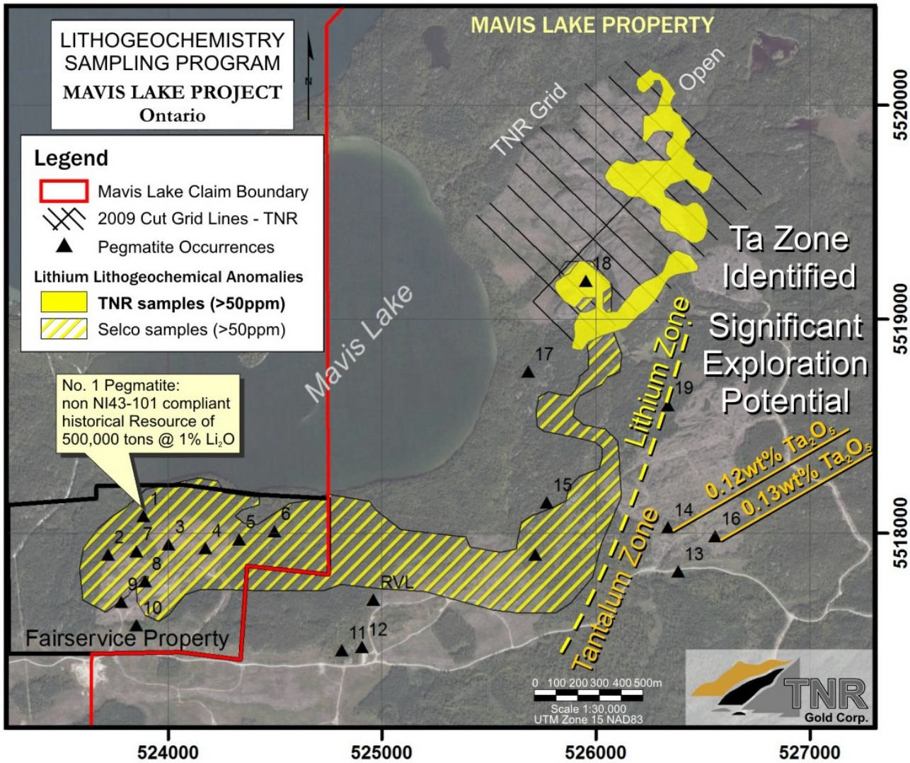
Figure 1: Lithium-Tantalum Zonation and Pegmatite Location Map – Mavis Lake and Fairservice Project, Ont.
