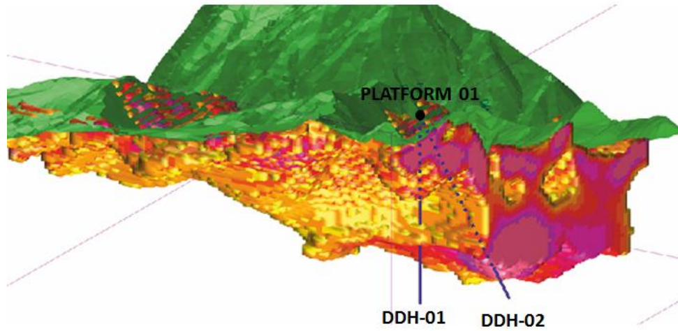
Isometric Model (3D) showing the morphology and interception of drill holes (DDH-01 and DDH-02) with the chargeability model at 300 meters depth.
