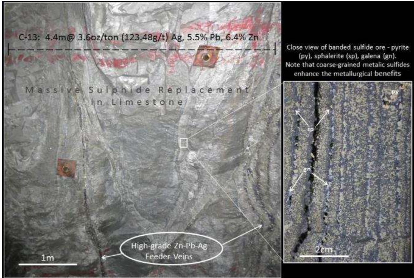
Figure 1: Underground Exposure (looking overhead) of the Rosa Zone (4510 level, sub-level 4) in Trevali's Santander Mine, Peru
