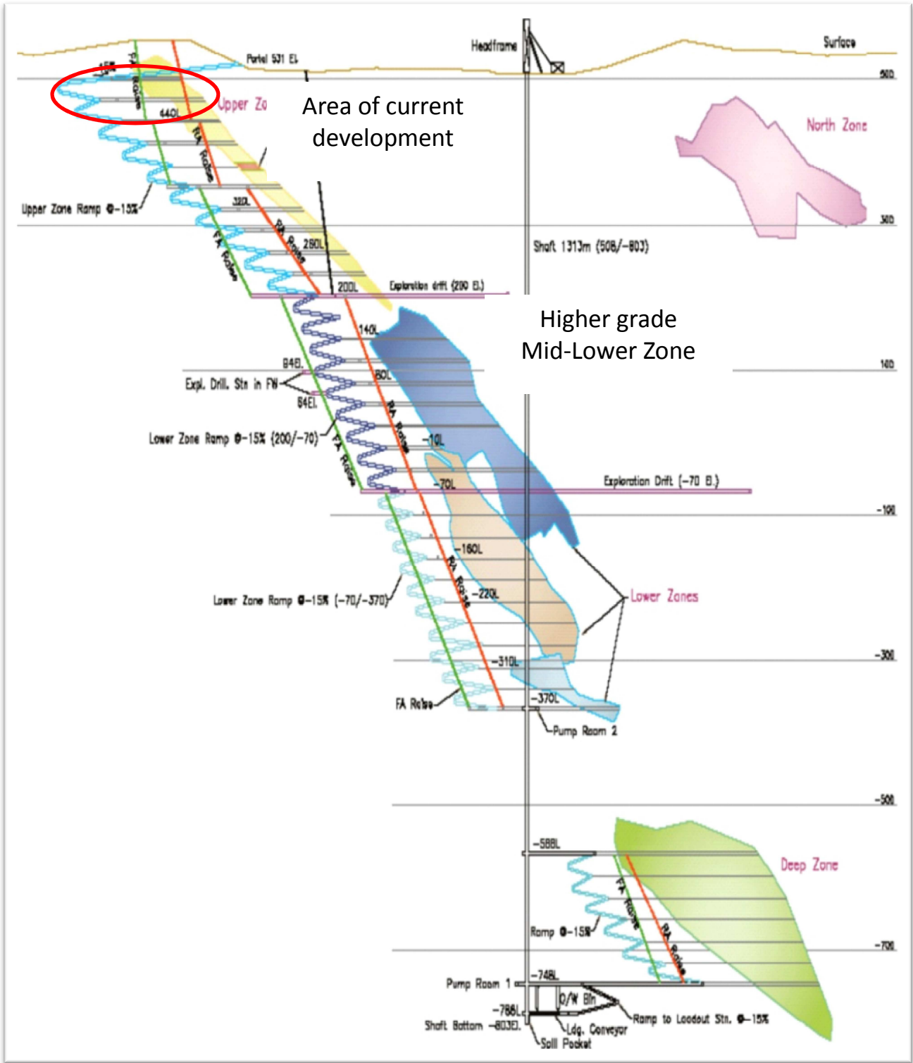
Figure 1: Cross-section of the Halfmile Deposit showing location of higher-grade zones
