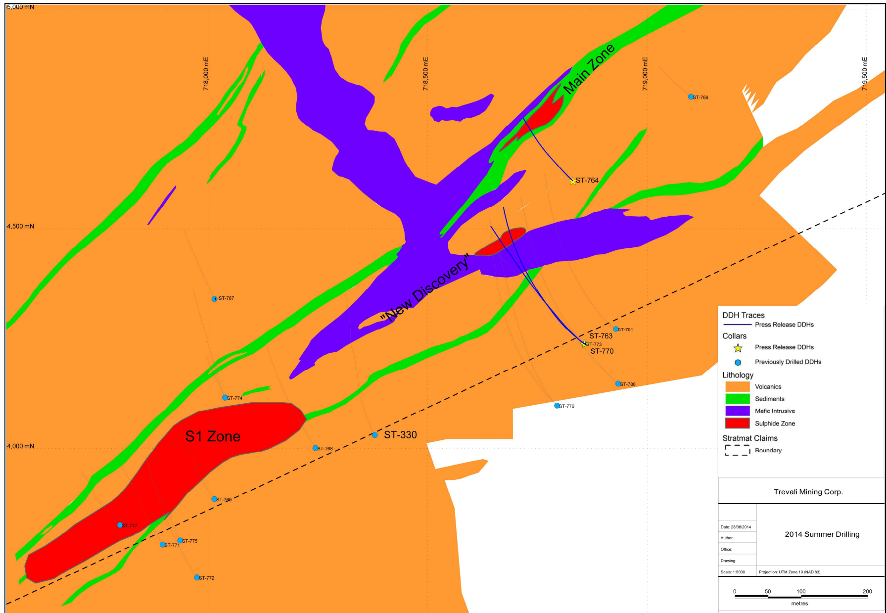
Figure 1: Stratmat Property map showing surface expression of mineralized zones and latest drill holes
