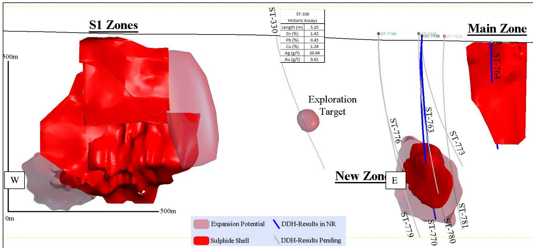
Figure 2: 3D long section view of the Stratmat Deposits looking N315°
