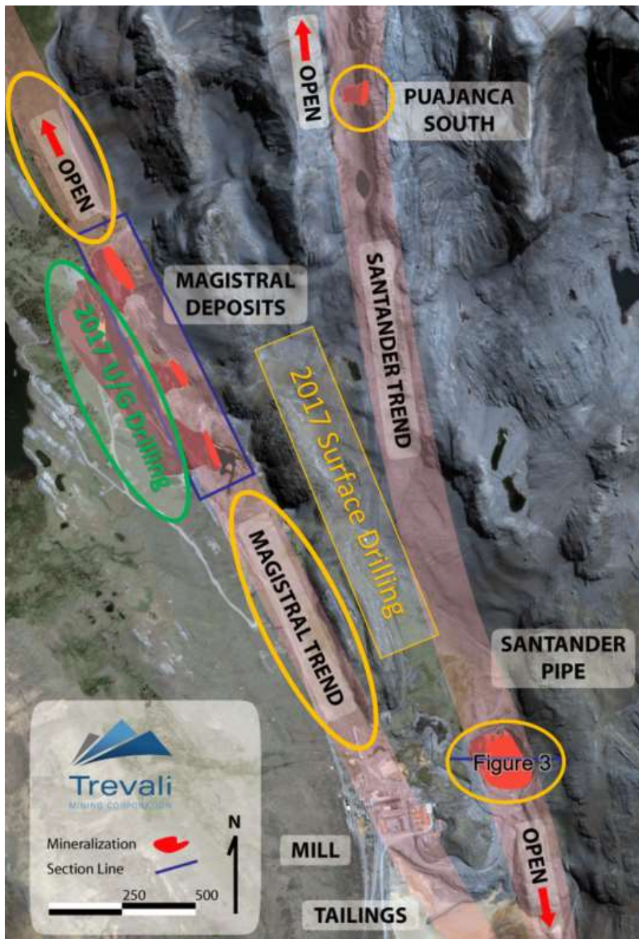
Figure 1: Map of the Santander property showing the Magistral deposits, the Santander Pipe target and a portion of Trevali’s 17-km long, prospective exploration trends.
